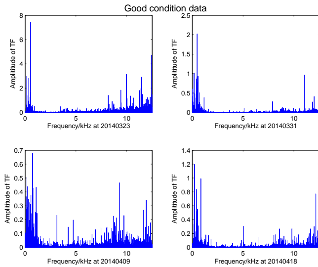
Fig. 17. TFs of good condition data collected at different times
