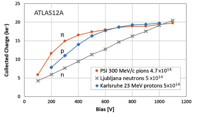
Fig. 9. Collected charge vs. bias of A12A samples irradiated with neutrons, protons, and pions to a fluence of 5 \times 10^{14} \text{ n}_{\text{eq}}/\text{cm}^2 .
