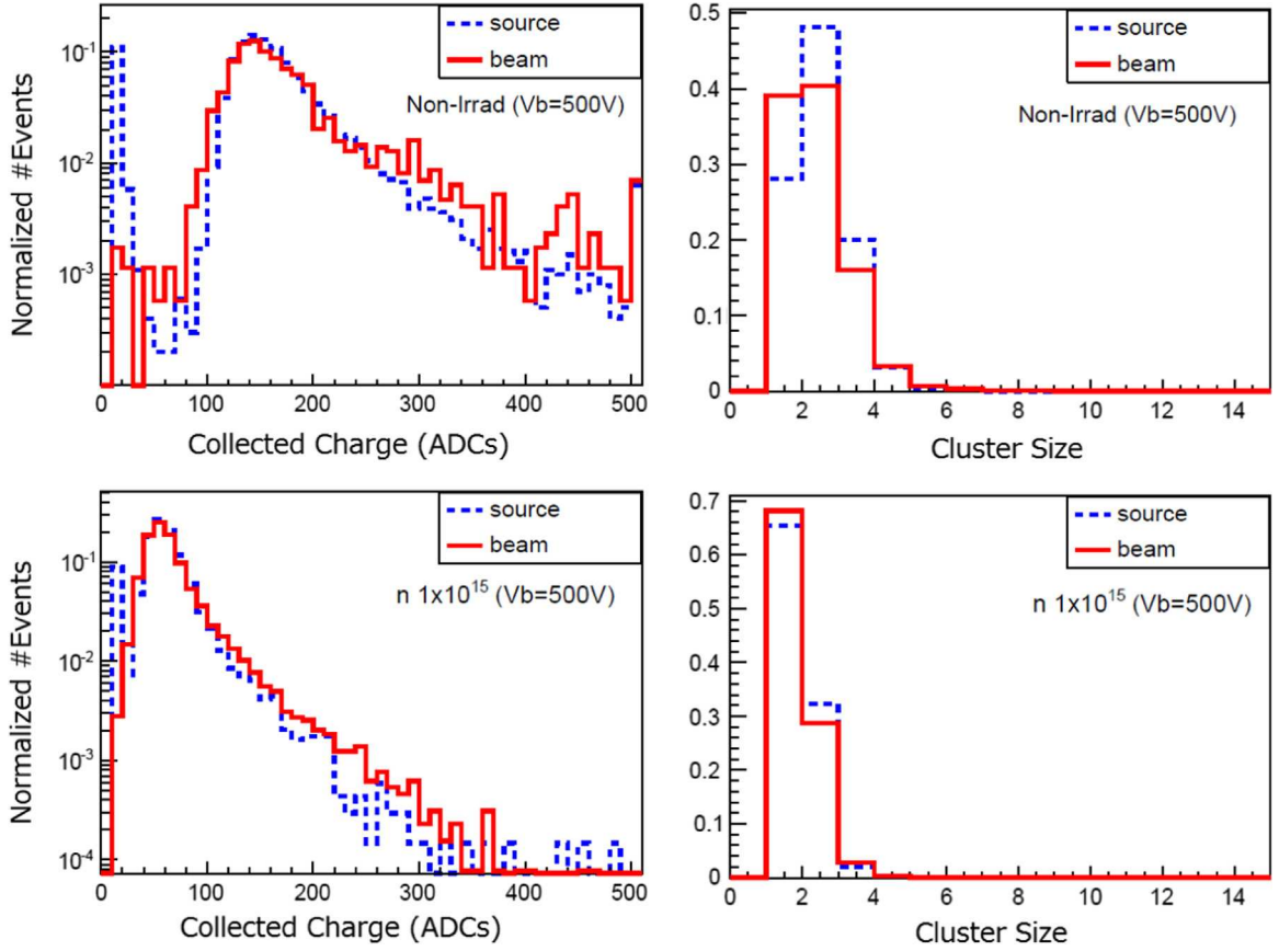
Fig. 7. Comparison of source (dashed) and beam (solid histograms) measurements of the non-irradiated (above) and 1 \times 10^{15} \text{ n}_{\text{eq}}/\text{cm}^2 irradiated samples (below). Comparison of charge distributions and cluster size distributions at 500 V.
