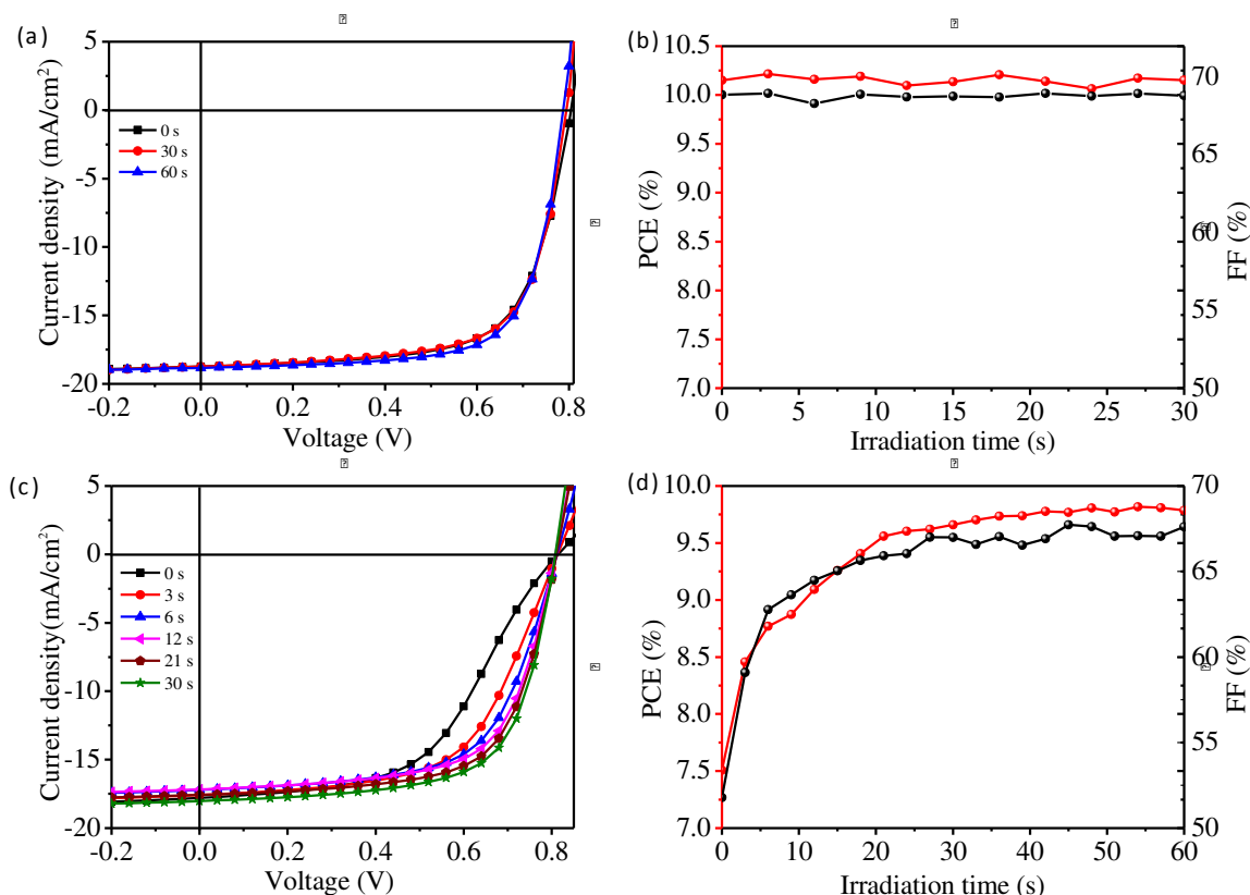
Figure 3. Light-soaking process of i-PSCs based on \text{TiO}_2\text{:TOPD} ETLs with and without UV and EA treatments. (a) J-V characteristics of inverted PSC device without light-soaking problem after UV and EA treatments, and (b) the corresponding evolution in PCE and FF as a function of irradiation time. (c) J-V characteristics of inverted PSC device with light-soaking issues without UV+EA treatments, and (d) the corresponding evolution in PCE and FF as a function of irradiation time.
