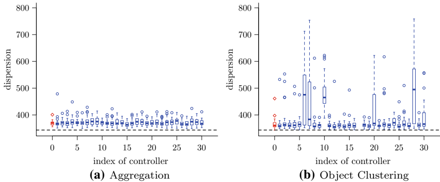
Fig. 6 a Dispersion of 50 simulated agents ( red box ) or replicas ( blue boxes ), executing one of the 30 inferred models in the aggregation case study. b Dispersion of 50 objects when using a swarm of 25 simulated agents ( red box ) or replicas ( blue boxes ), executing one of the 30 inferred models in the object clustering case study. In both (a) and (b) , boxes show the distributions obtained after 400 s over 30 trials. The models are from the 1000th generation. The dashed black lines indicate the minimum dispersion that 50 individuals/objects can possibly achieve (Graham and Sloane 1990). See Sect. 4.3 for details (Color figure online)
