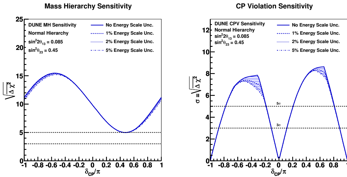
Figure 3.24: Expected sensitivity of DUNE to determination of the neutrino mass hierarchy (left) and discovery of CP violation, i.e. \delta_{CP} \neq 0 or \pi , (right) as a function of the true value of \delta_{CP} , assuming equal running in neutrino and antineutrino mode, for a range of values assigned to the “a” parameter in the energy-scale variation described in the text. In the MH figure, the case with no energy-scale systematic provides a significance of at least \sqrt{\Delta\chi^2} = 5 for all values of \delta_{CP} . In the CPV figure, the case with no energy-scale systematic provides a significance of at least 3\sigma for 75% of \delta_{CP} values. (See Figures 3.8 and 3.14 for the possible range of exposures to achieve this level of significance.) Sensitivities are for true normal hierarchy; neutrino mass hierarchy and \theta_{23} octant are assumed to be unknown.
