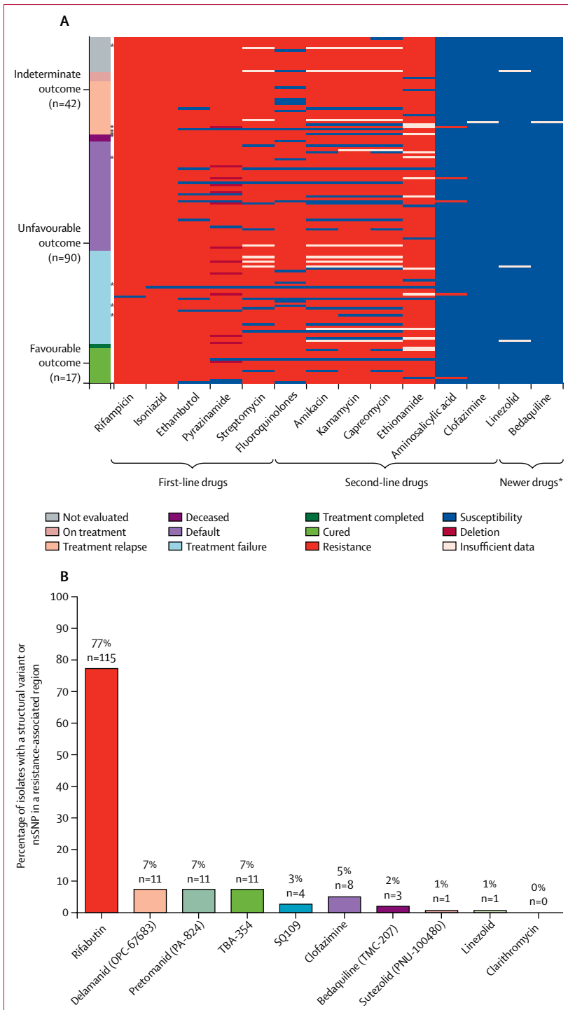
Figure 3: Genome-based analysis of polymorphisms predictive of resistance to antituberculosis drugs
