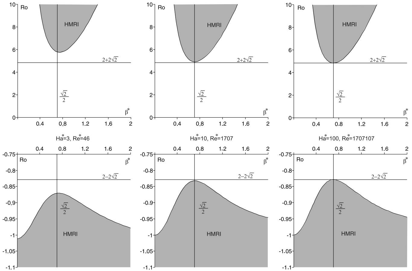
Figure 4. Inductionless approximation ( Pm = 0 ): two domains (Equation (57)) of HMRI (gray) are within the bounds (Equation (67)). It is seen how the scaling law (Equation (68)) works. HMRI is possible even for Pm = 0 —the paradox of inductionless magnetorotational instability (Priede et al. 2007).
