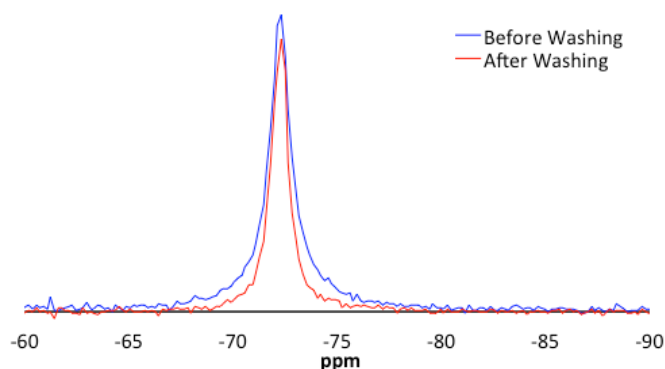
Figure 2. ^{19}\text{F} NMR spectra of thiol-acrylate polyHIPE containing 50% TMPTMP functionalized with HFIPA by a UV initiated reaction, before (dark trace) and after washing with THF.
