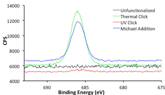
Figure 3. High resolution F(1s) 29 XPS spectra of HFIPA-functionalized thiol-acrylate polyHIPEs containing 50% TMPTMP. From top to bottom: thermal click reaction; Michael addition reaction; unfunctionalized sample; UV click reaction.
