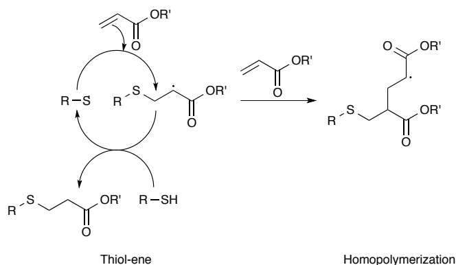
Scheme 1. Competing reactions occurring during network formation between thiols and acrylates: thiol-ene reaction (left cycle); and acrylate homopolymerization (right)
