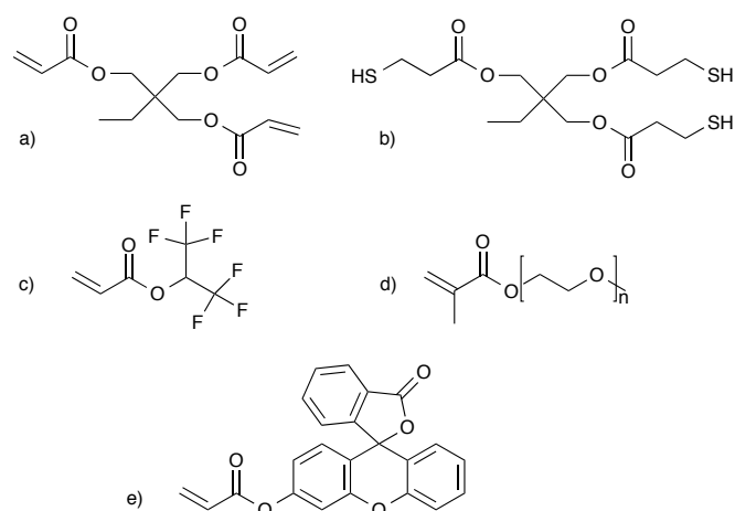
Figure 1. Chemical structure of the monomers used to prepare and functionalize thiol-acrylate polyHIPEs. a) trimethylolpropane triacrylate (TMPTA), b) trimethylolpropane tris(3-mercaptopropionate) (TMPTMP), c) hexafluoroisopropyl acrylate (HFIPA), d) poly(ethylene glycol) methyl ether methacrylate (PEGMA), e) fluorescein O -acrylate (FA).
