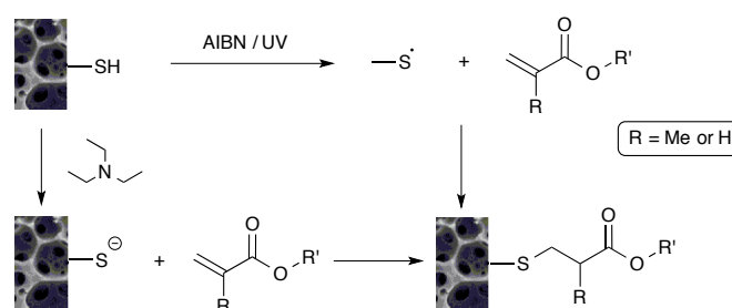
Scheme 3. Functionalization of residual thiols by radical-mediated “click” and Michael addition reactions.
