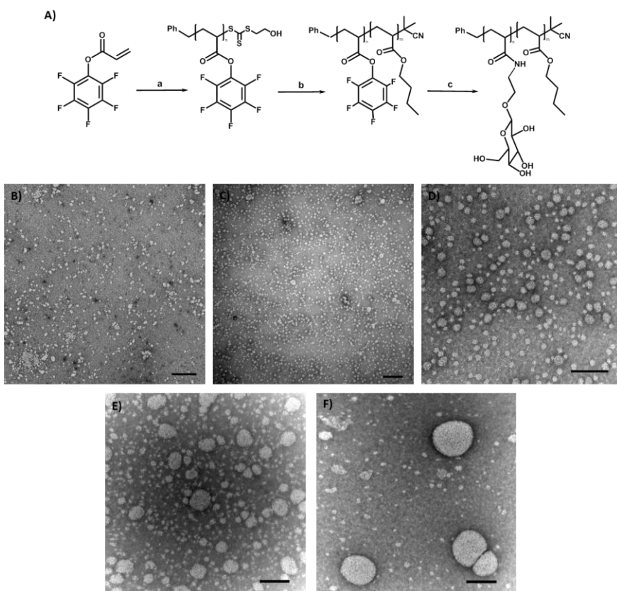
Figure 1. A) Schematic representation of amphoteric glycopolymers synthesis (Conditions: a) BHECTT and AIBN in benzene at 70 °C for 6 h, b) BA and AIBN in benzene at 70 °C for 6 h followed excess AIBN at 70 °C for 6 h, c) 2'-aminoethyl- \beta -D-glucopyranoside and TEA in DMF-water at 30 °C for 18 h. B)-F) TEM images of glyco-NPs made from B) p(N \beta GlcEAM) 15 -
