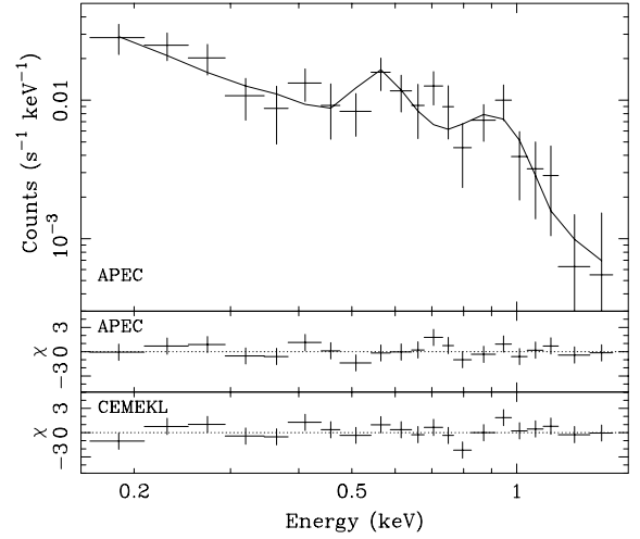
Figure 2. The XMM-Newton EPIC-pn spectrum of TRAPPIST-1 fitted with our two temperature APEC model (top). The middle panel shows the normalised residuals to this fit, while the bottom panel shows the residuals to our fit with the cemekl model.
