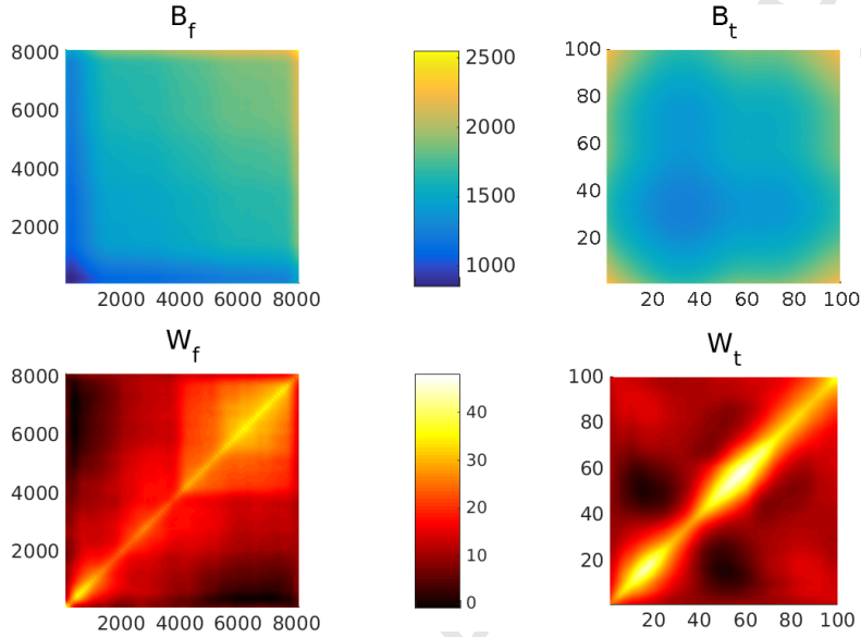
Figure 2: Sample between-language and within-language covariances of speech data for frequency and time directions. There is a clear ridge along the diagonal of the within-group covariances indicating that similar times and frequencies are highly positively correlated. The higher correlations in the high frequencies of the within-group frequency covariance are associated with recordings at lower audio sampling rates capturing fewer details in these ranges of frequencies. Rerunning the analyses performed in Section 5 whilst excluding these higher frequencies produces broadly similar results. Alternatively, excluding observations with low sampling rates has been examined in [66, Section 7.1] with both analyses leading to the same conclusion regarding tree-amenability.
