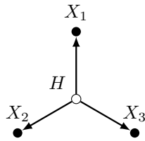
Figure 5: Tripod tree. A strictly trivalent tree with n_\ell leaves contains \binom{n_\ell}{3} conditional independence relationships which can each be expressed as a tripod tree.
