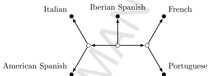
Figure 9: Topology of UPGMA generated tree for the second component.
