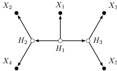
Figure 6: Five leaf tree.
