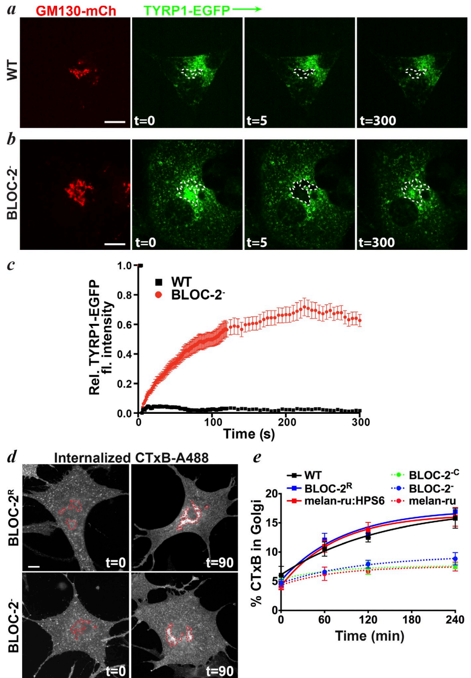
Figure 6. Retrograde trafficking of TYRP1 to the Golgi is specifically increased in BLOC-2 - melanocytes. (a–c) WT melan-Ink4a or BLOC-2 - cells transiently expressing TYRP1-EGFP and GM130-mCh to mark the Golgi, were pre-treated with CHX for 60 min at 37°C and then imaged by spinning disk microscopy ( t = 0). GFP fluorescence within the Golgi region labeled by GM130-mCh was bleached at frame 5 ( t = 5), and recovery of TYRP1-EGFP fluorescence intensity was quantified over time by normalizing to prebleach GFP intensity of the same region. (a and b) Representative images for GM130-mCh and TYRP1-EGFP from t = 0, t = 5, and t = 300 (300 s) for WT (a) and BLOC-2 - cells (b). Bleached region is indicated by the dotted white line in TYRP1-EGFP images. Bars, 10 μm. (c) Quantification of fluorescence recovery. Rel., relative; fl., fluorescence. Values represent the means ± SD of GFP intensity traces of 15 cells of each type. (d and e) WT (melan-Ink4a), “rescued” BLOC-2 R (melan-coa:hHPS3), or melan-ru: HPS6, or BLOC-2-deficient BLOC-2 - (melan-coa), BLOC-2 -C , or melan-ru cells on coverslips were incubated with AF488-conjugated CTxB on ice for 1 h and then at 20°C for 15 min to allow for internalization. Cells were washed once and incubated at 37°C for the indicated times, fixed, labeled with the anti-giantin antibody and analyzed by IFM. (d) Representative CTxB fluorescence images of BLOC-2 R and BLOC-2 - cells at the 0 and 90 min time points ( t = 0, t = 90) showing appearance of CTxB in the Golgi (giantin staining; red outline) by 90 min. Bar, 10 μm. (e) Fluorescence intensity of AF488-CTxB in the giantin-positive region was quantified and plotted over time for all cell types. Values (means ± SD) for all BLOC-2-deficient lines are significantly different ( P < 0.01 at 60 min and P < 0.001 at 120 and 240 min) from their paired BLOC-2-sufficient lines.
