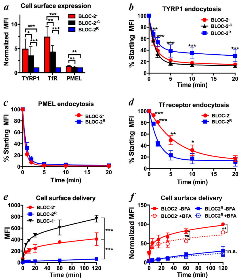
Figure 4. Increased TYRP1 cycling through the plasma membrane in BLOC-2 - melanocytes. (a) Comparison of cell surface levels of TYRP1, TfR, or PMEL among BLOC-2 - , BLOC-2 -C , and BLOC-2 R melanocytes by flow cytometry after labeling of whole cells on ice with unlabeled primary and AF488-conjugated secondary antibody. The mean fluorescence intensity (MFI) \pm SD over 4–15 experiments, each performed in duplicate or quadruplicate, was normalized to 1.0 for BLOC-2 R melanocytes within each experiment. (b–d) Quantification of TYRP1 (b), PMEL (c), and TfR (d) endocytosis rates. BLOC-2 - , BLOC-2 -C , or BLOC-2 R cells were incubated with unlabeled antibodies on ice and loss of surface antibody (detected with fluorescent secondary antibody) over time at 37°C was quantified by flow cytometry. MFI at each time point was calculated and plotted relative to MFI at time 0 (defined as 100%). Values (means \pm SD) were from two to eight separate experiments performed in duplicate. (b and d) P-values are indicated for comparison of BLOC-2 R to BLOC-2 - cells. Values in c were not significantly different. (e and f) Quantification of TYRP1 flux through the plasma membrane. Uptake of saturating levels of fluorescent anti-TYRP1 antibody by BLOC-2 - , BLOC-2 R , or BLOC-1 - deficient melan-mu cells (BLOC-1 - ) at 37°C was quantified over time by flow cytometry. In f, cells were left untreated or were treated with 10 \mu g/ml brefeldin A (BFA) for 1 h before and during the experiment as indicated. Values (means \pm SD) were from at least three independent experiments performed either in duplicate or quadruplicate and represent raw MFI (e) or a normalized value (f) calculated as the percentage of the MFI value for untreated BLOC-2 - cells at 2 h. P-values shown in e correspond to all points in the graph except the initial time point; p-values in f are shown only for differences deemed significant between -BFA and +BFA samples. *, P < 0.05 ; **, P < 0.01 ; ***, P < 0.001 ; n.s., not significant.
