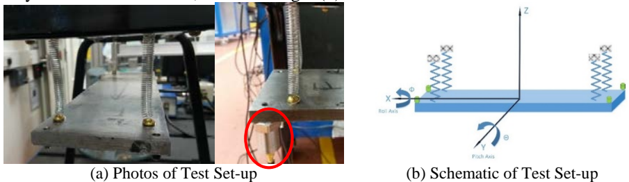
Fig. 2 Test Set-up
