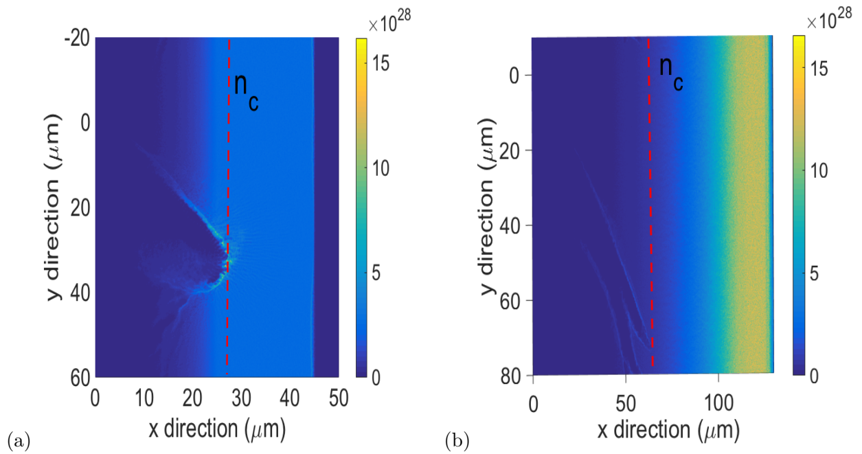
FIG. 8. An example of electron density values colour-coded in units of \text{m}^{-3} after 0.55 ps with a) 5 \mu\text{m} , b) 15 \mu\text{m} scale length as simulated by the EPOCH 2D PIC code. The dashed vertical line indicates the critical density surface. The laser radiation is incident at 40^\circ to the target normal.
