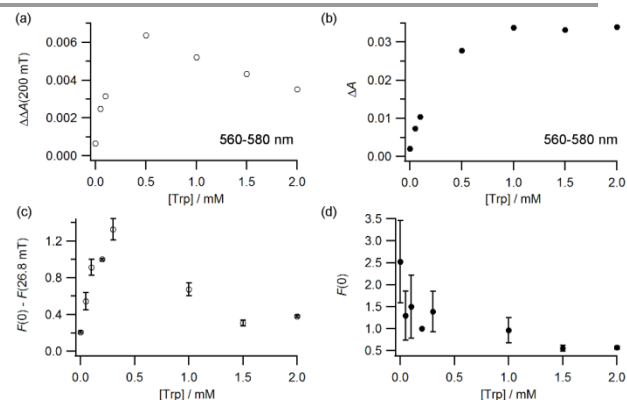
Fig. 3 Comparison of absorption- and fluorescence-detected MFEs. (a) Transient absorption difference signal, \Delta\Delta A = \Delta A(200 \text{ mT}) - \Delta A(0) . (b) Transient absorption signal in the absence of a magnetic field, \Delta A(0) . (c) Fluorescence difference signal F(0) - F(26.8 \text{ mT}) . (d) Initial fluorescence intensity in the absence of a magnetic field. The data in panels (a) and (b) are averages over the wavelength range 560–580 nm and the time period 5–10 \mu\text{s} . The data in panels (c) and (d) have been normalised to the measurement at 200 \mu\text{M} Trp and error bars show SEM. The FAD concentrations were 0.2 mM (absorbance) and 1 \mu\text{M} (fluorescence).
