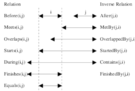
■ Figure 2 Allen's Interval Algebra Base Relations
