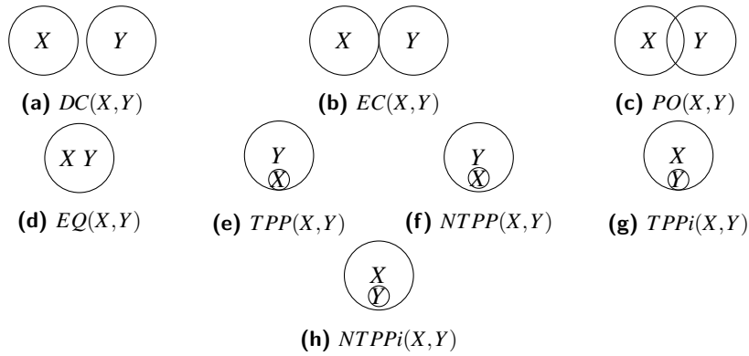
■ Figure 1 RCC-8 Base Relations
