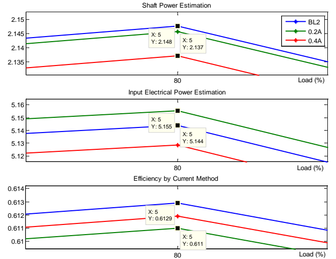
Fig. 10 Motor efficiency calculations at 80% loading
