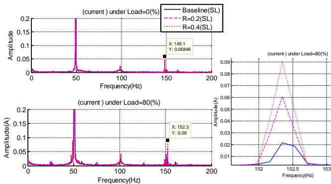
Fig. 12 Frequency spectral plot of motor current signals under 0% and 80% load.
