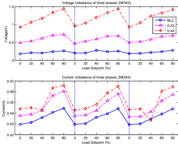
Fig. 9 Voltage and current imbalances under NEMA definitions
