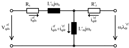
Fig.7 Induction motor steady state equivalent circuit
