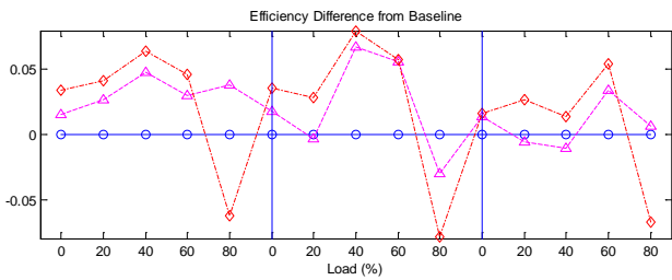
Fig. 11 Motor efficiency calculations using air gap torque method
