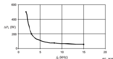
Fig. 1 Losses of motor due to switching frequency [2]
