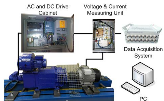
Fig. 3 Laboratory Test Rig
