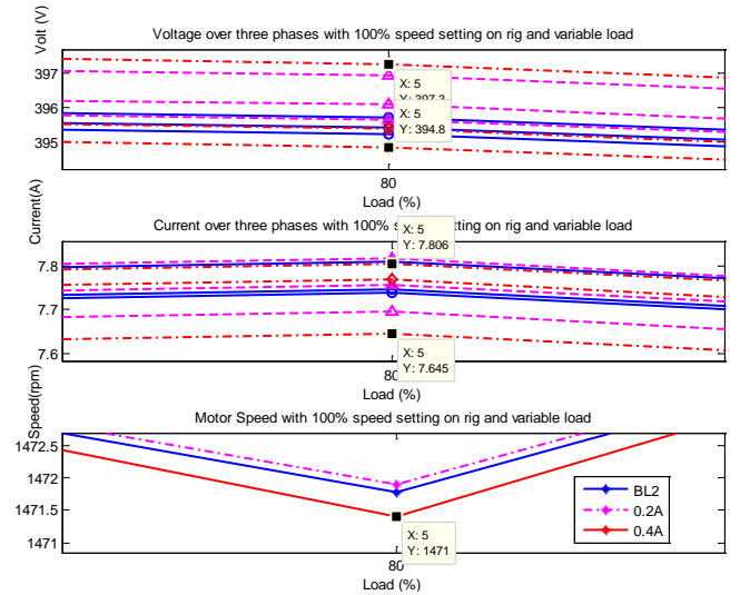
Fig. 8 Plot of voltage, current and speed over 3 phases at 80% load condition with 100% speed setting. BL2 = Baseline (Healthy Motor); 0.2A = Stator Resistance imbalance of 0.2Ω; 0.4A = Stator Resistance imbalance of 0.4Ω.
