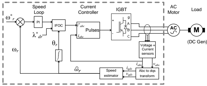
Fig. 6 Inverter FOC diagram
