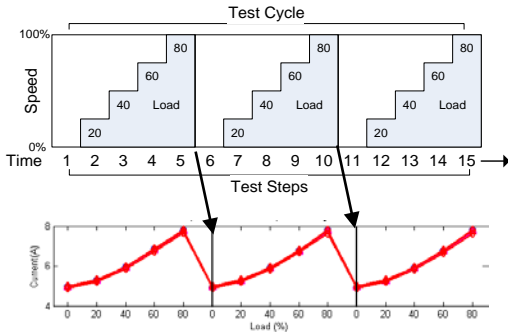
Fig. 4 Test cycle and example plot
