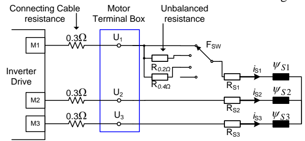
Fig. 5 Motor magnetising circuit detailing the stator phase resistance fault inserted in one of the three phase connections internally in the motor on phase 1 (STAR circuit)
