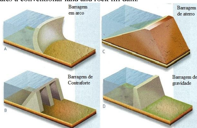
Figure 1. Types of dams according to the material used. Source: Adapted from AUSTRALIAN GEOGRAPHIC 1
