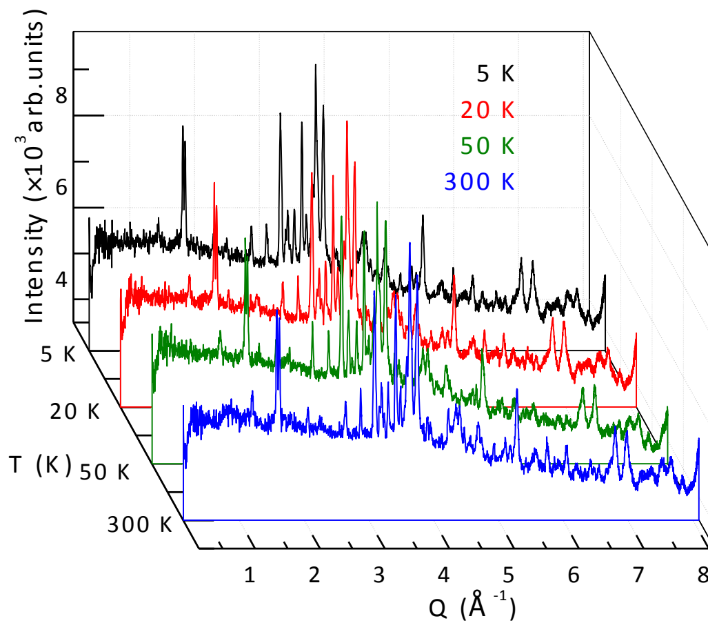
FIG. 7. A series of neutron powder diffraction patterns for Na-birnessite obtained at 5, 20, 50 and 300 K. The absence of reflections of magnetic origin in the low-temperature region, indicates that no long-range magnetic order develops below 29 K.
