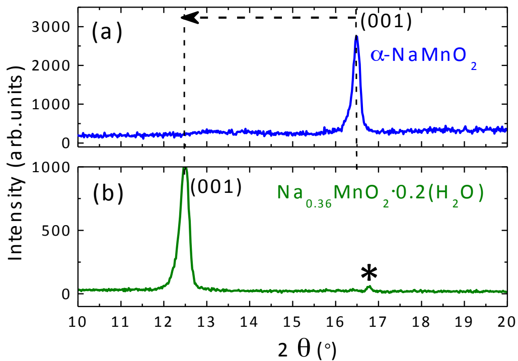
FIG. 3. Low-angle part of the XRPD patterns for \alpha\text{-NaMnO}_2 (a) and the Na-birnessite (b), showing the characteristic shift of the 001 Bragg reflection upon hydration; (*), non-converted parent \alpha\text{-NaMnO}_2 .
