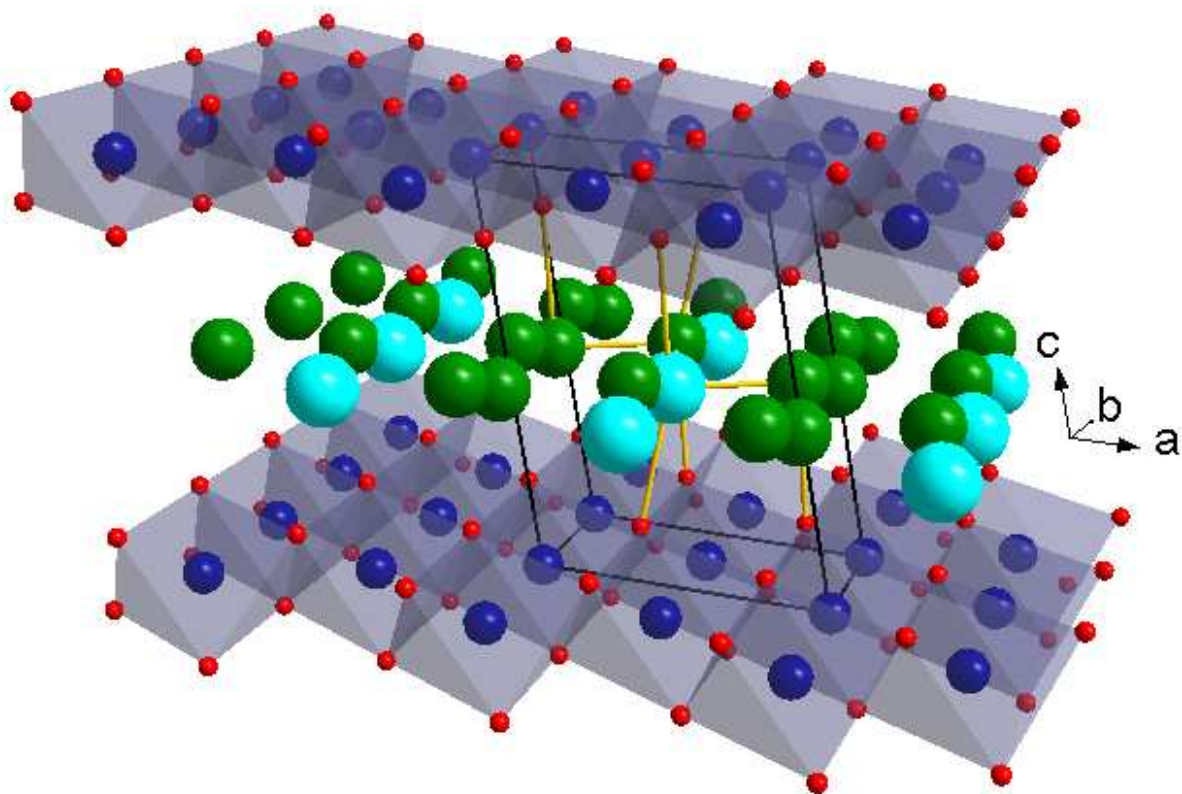
FIG. 4. Schematic representation of the crystal structure of the Na-birnessite: the manganese, oxygen, sodium atoms are represented with the blue, red and green spheres; the H 2 O molecules in the interlayer space are shown with the turquoise spheres; cell-edges are represented with the black lines. For ease of visualization, Na atoms and H 2 O molecules, occupying identical positions in the reported structure, are displayed in alternating positions in the model (ICSD 262208).
