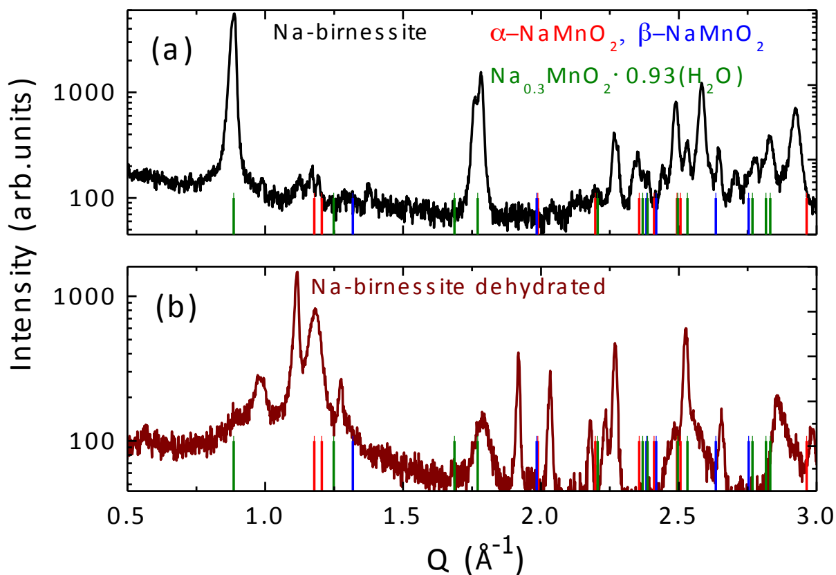
FIG. 6. Comparison of the XRPD patterns of the Na 0.3 MnO 2 ·0.2H 2 O birnessite's polycrystalline powder (a) and the dehydrated compound (b) taken after the TGA experiment performed up to 1100° C. Indexing of the reflections has been done on the basis of the \alpha -NaMnO 2 (ICSD 16270), \beta -NaMnO 2 (ICSD 16271) and the Na 0.3 MnO 2 ·0.93H 2 O (ICSD 262208) phases, whose Bragg reflections are indicated with red, blue and green tick marks, respectively. Bragg peaks attributed to the Mn 3 O 4 (ICSD 68174, ICSD 1514104) are left without tick marks for ease of comparison.
