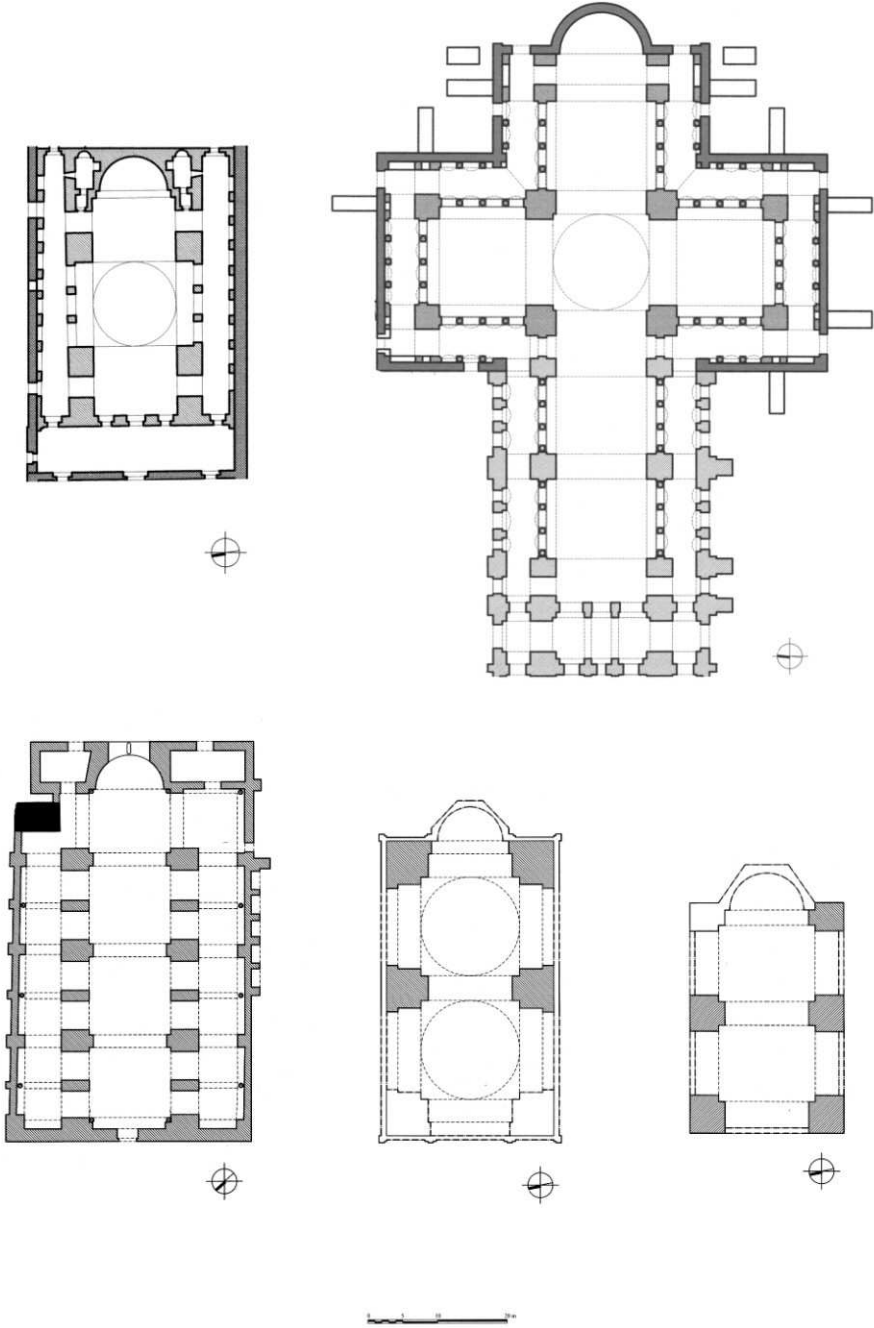
Fig. 1: The Early Byzantine Vaulted Churches of West Asia Minor, Table of Plans. Upper row, left to right: St. Mary at Ephesos and St. John at Ayasuluk. Bottom row, left to right: “Urban Basilica” at Hierapolis, St. John at Philadelphia and Building D at Sardis (CAD drawings by Carolina Vasilikou, 2009).
