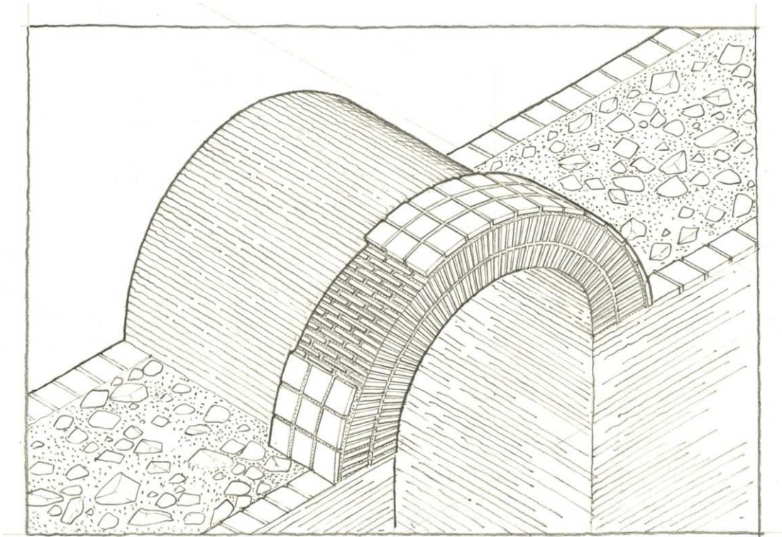
Fig. 9: Ephesos, St. Mary, Cross-domed Church, detail of barrel vault connecting the two parts of the northwest pier (pencil on paper, Nikolaos Karydis, 2009).
