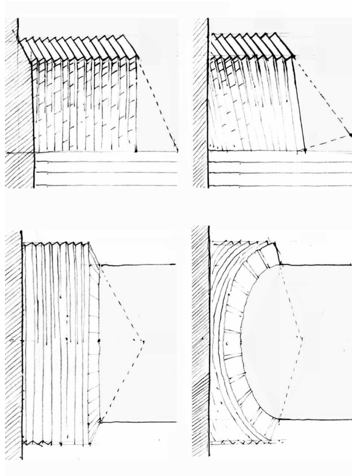
Fig. 6: Two Types of Barrel Vaults Made of Pitched Bricks, interpretive plans and sections (pencil on paper, Nikolaos Karydis 2003, after Auguste Choisy 1883).
