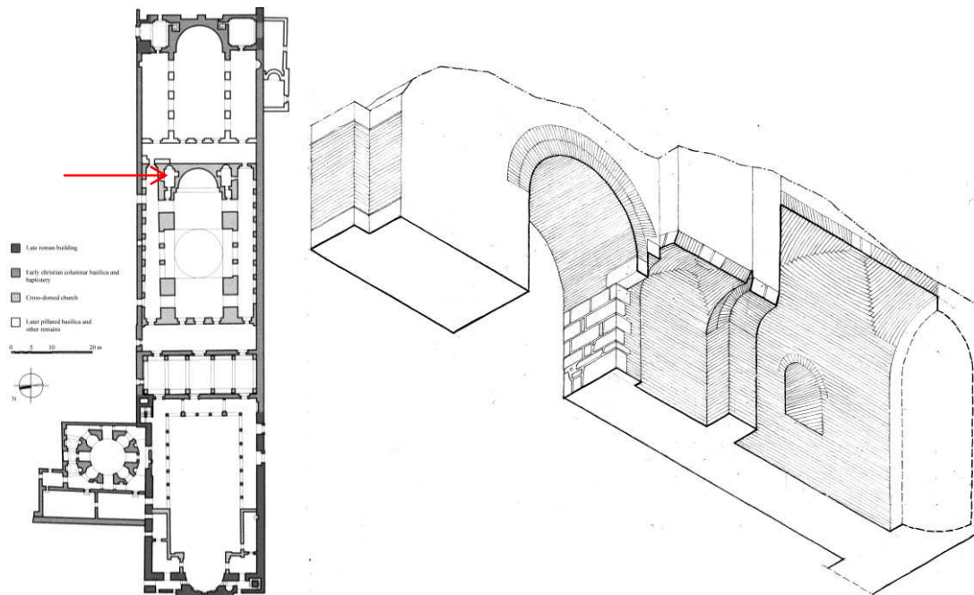
Fig. 12: Ephesos, St. Mary, Cross-domed Church, axonometric drawing of the secondary vaults covering the north side-chamber (pencil on paper, Nikolaos Karydis, 2009).
