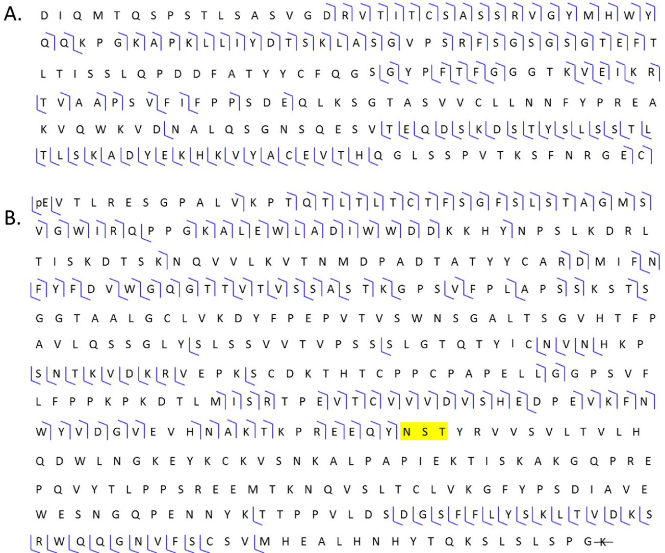
Fig. 3. Amino acid sequence coverage for (A) IgG1 mAb light chain and (B) heavy chain determined by a combination of MALDI-MS/MS and middle-down ETD analyses. The overall sequence coverage was 35.9% and 52.6% for the heavy and light chains, respectively. Glutamine (Q) to pyroglutamate (pyroGlu, pE) conversion and C-terminal lysine truncation were detected on the heavy chain. One glycosylation site is highlighted in yellow.
