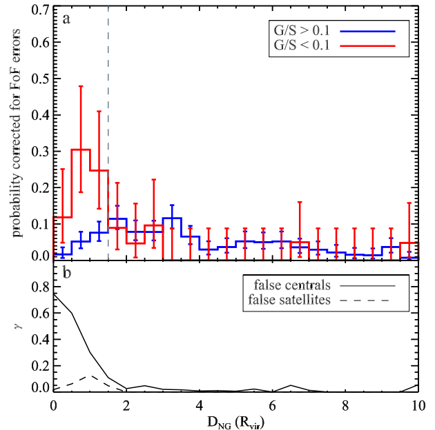
Figure 8. (a) Normalized probability distribution of the distances of M_h < 10^{11.4} M_\odot centrals from the nearest M_h > 10^{12} M_\odot group with recession velocity difference < 500 \text{ km s}^{-1} . Distances are given as a multiple of R_{\text{vir}} of the nearest M_h > 10^{12} M_\odot group. Uncertainties come from Poisson statistics. The gas-poor population shows a preference to be found within \sim 1.5R_{\text{vir}} of the nearest M_h > 10^{12} M_\odot group. The gray dashed line shows the maximum “splashback radius” proposed by More et al. (2015) as a more physical definition of halo boundaries. (b) Errors on central/satellite designation in FoF group finding. The solid line indicates the fraction of galaxies classified as centrals in M_h < 10^{11.4} M_\odot halos that are truly satellites of M_h > 10^{12} M_\odot halos. The dashed line indicates the fraction of satellites in M_h > 10^{12} M_\odot halos that are truly centrals in M_h < 10^{11.4} M_\odot halos. These corrections are already applied to panel (a).
