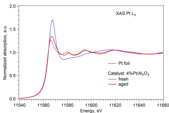
Figure 2. Pt L_3 -edge XAS spectra of freshly prepared and aged 4%Pt/Al 2 O 3 diesel oxidation catalysts measured in transmission mode at CAT-ACT. The spectrum of a Pt foil was measured as reference and for energy calibration and is shown for comparison.
