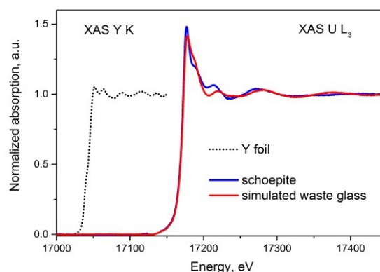
Figure 3. U L_3 -edge XAS spectra of U(VI) or ‘uranyl’ species in the mineral meta-schoepite (UO 3 · nH 2 O) and a simulated U-borosilicate nuclear waste glass (4.7 wt.% UO 2 loading). Y metal was measured as energy calibration standard.
