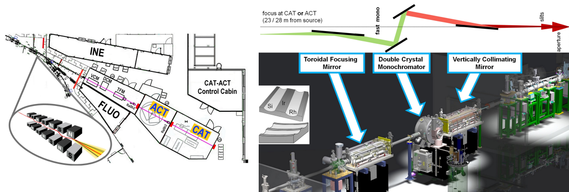
Figure 1. Layout of the CAT-ACT beamline at ANKA with two in-line experimental stations (left). CAT-ACT optical components designed and manufactured by FMB Oxford (Oxford, United Kingdom). From right to left: frontend components (intensity absorber, X-ray beam position monitor, white beam slit), collimating mirror, double crystal monochromator, diagnostics module, toroidal focusing mirror, beam shutter separating ACT hutch from optics section. Inset: focusing mirror coating scheme.
