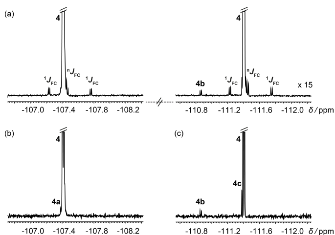
Fig. 3. (a) ^1\text{H} decoupled ^{19}\text{F} spectrum of a degraded sample of the antifungal drug fluconazole ( 4 ); (b), (c) ^1\text{H} decoupled, ^{13}\text{C} isotopomer-suppressed ^{19}\text{F} spectra acquired separately for each parent signal using the pulse sequence of Fig. 2 with selective ^{19}\text{F} 180^\circ pulses.
