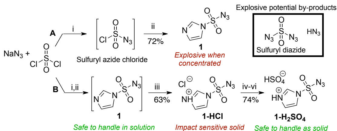
Scheme 1. Reported syntheses of imidazole-1-sulfonyl azide, 17 HCl and H 2 SO 4 salts. a
