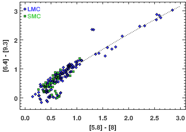
FIG. 18.— The relationship between [6.4]-[9.3] and [5.8]-[8] colors and a quadratic fitted to data with [6.4]-[9.3] > 0.35 . The two data points at [6.4]-[9.3] \sim 2.3 and [5.8]-[8] \sim 1.3 are badly mispointed, resulting in artificially red [6.4]-[9.3] colors, which have been replaced in the data tables using estimates from the fitted relation (see text).
