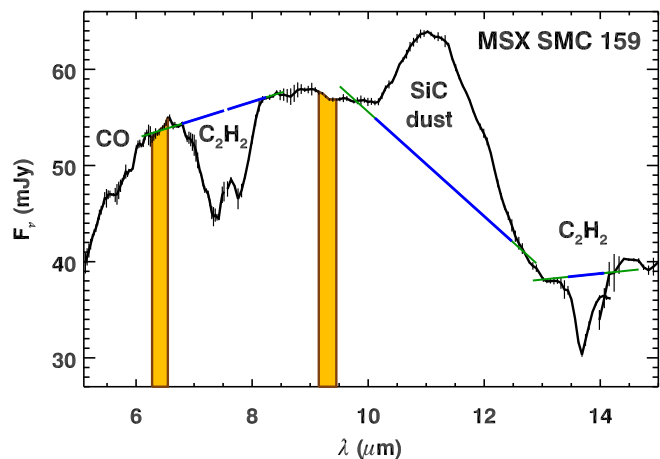
FIG. 1.— The Manchester method applied to the 5–15 \mu\text{m} spectrum of MSX SMC 159. The [6.4]–[9.3] color provides an estimate of the relative contributions of stellar photosphere and amorphous carbon dust in two spectral regions relatively free of absorption or emission features. Line segments are used to estimate the continuum under or over the \text{C}_2\text{H}_2 absorption band at 7.5 \mu\text{m} , the Q branch of the \text{C}_2\text{H}_2 band at 13.7 \mu\text{m} , and the SiC dust emission feature at \sim 11.3 \mu\text{m} .
