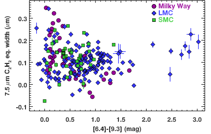
FIG. 8.— The strength of the 7.5 \mu m C 2 H 2 absorption band versus [6.4]–[9.3] color.
