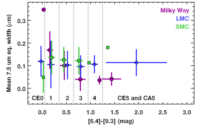
FIG. 9.— The strength of the 7.5 \mu m C 2 H 2 absorption band versus [6.4]–[9.3] color, binned by CE class to illustrate the general trends in the data. When determining means, negative equivalent widths have been treated as zero, because acetylene emission is unlikely.
