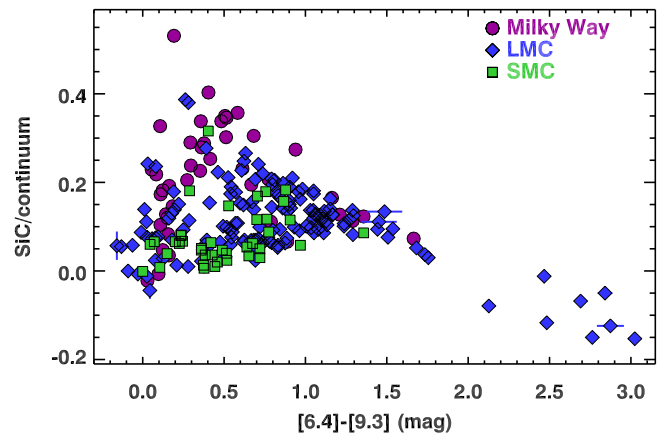
FIG. 5.— The strength of SiC dust emission as a function of [6.4]-[9.3] color. As the [6.4]-[9.3] color increases, stars follow one of two tracks. The SiC strength increases quickly in more metal-rich stars, then turns over and decreases. In metal-poor stars, the SiC strength increases more gradually. Most of the stars with [6.4]-[9.3] \gtrsim 1.5 have negative SiC strengths, indicating absorption.
