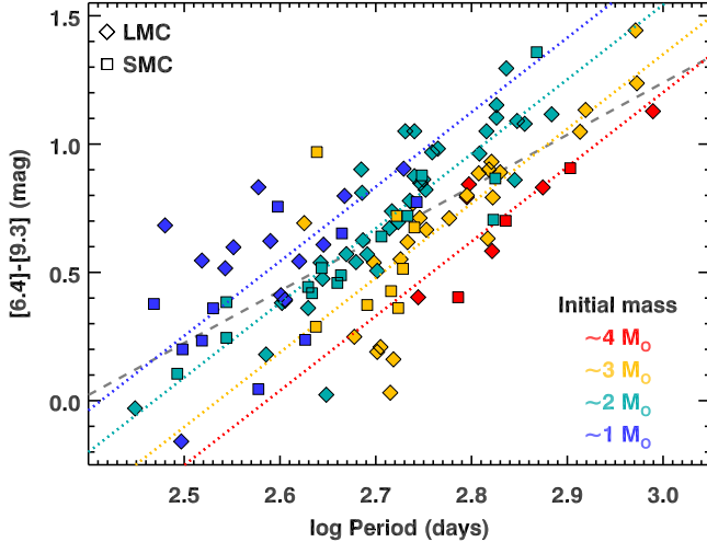
FIG. 11.— The [6.4]-[9.3] color as a function of pulsation period with the Magellanic sample, color-coded by their initial mass as estimated from their bolometric magnitude. Sources not assigned to a mass bin are not included. The width of the relation between [6.4]-[9.3] color and period clearly arises from the mass distribution of the samples. The gray dashed line is a line fitted to all of the data, while the colored dotted lines are fitted to each mass bin separately (see Section 4.3).
