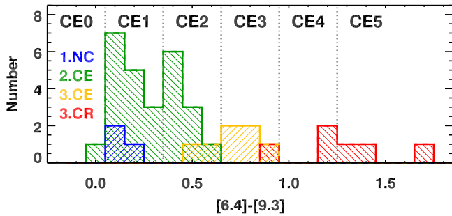
FIG. 3.— The distribution of the Galactic carbon stars in our control sample with [6.4]-[9.3] color, segregated by their infrared spectral classifications from Kraemer et al. (2002). The [6.4]-[9.3] color increases nearly monotonically along the sequence 1.NC–2.CE–3.CE–3.CR.
