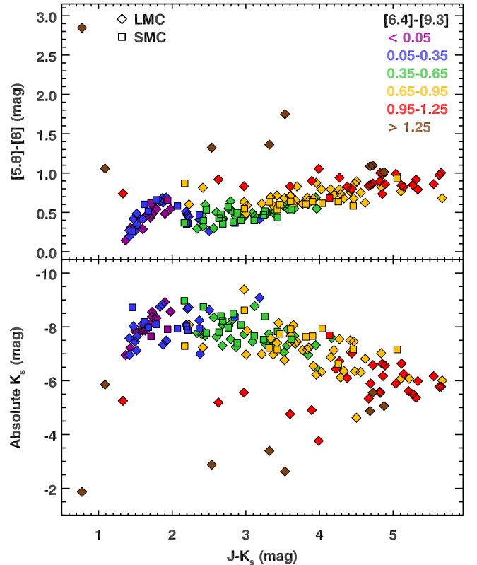
FIG. 12.— Color-color and color-magnitude diagrams featuring the J-K_s colors on the horizontal axis. Symbols are coded for galaxy with shape and for [6.4]-[9.3] color with color. The [6.4]-[9.3] intervals correspond to the CE0–5 classifications. None of the CE5s and only about half of the CE4s follow the sequences. (CE4: 0.95 < [6.4]-[9.3] < 1.25 ; CE5: [6.4]-[9.3] > 1.25 .)
