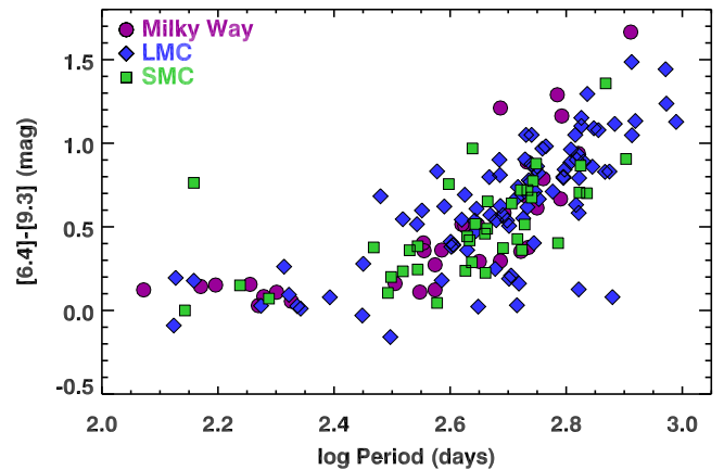
FIG. 4.— The [6.4]-[9.3] color of the carbon stars in the Galaxy, LMC, and SMC as a function of pulsation period. For periods \gtrsim 250 days, the colors generally grow redder with longer periods, but with considerable scatter. No dependency on metallicity is apparent.
