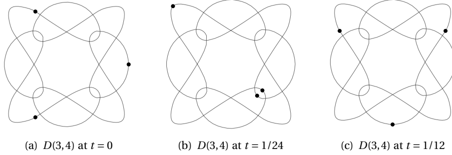
FIGURE 2.2: A choreography for the 3-body problem with 4-fold symmetry (“3 particles on a Celtic knot”). Note that the particles at t = 1/12 are obtained from those at t = 0 by rotating by -\pi/2 and relabelling by \sigma_1^{-1} = (1\ 3\ 2) . This corresponds to the symmetry element g = (R_{3\pi/2}, \sigma_1^2, 1/12) , the generator of C(3,4) . Fig. (a) demonstrates the element (\kappa, (2\ 3), \bar{0}) \in D(3,4) , while Fig. (b) illustrates (\kappa_{\pi/4}, (1\ 3), \bar{1}/12) and Fig. (c) illustrates (\kappa_{\pi/2}, (1\ 2), \bar{1}/6) . See [27] for the animation.
