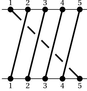
FIGURE 5.1: The braid \delta for n = 5 . One has \pi(\delta) = (1\ 2\ 3\ 4\ 5) = \sigma_1 .
