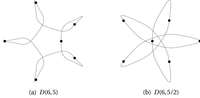
FIGURE 2.1: Comparison of different values of \ell : D(6,5) and D(6,5/2) is the difference between the symmetries of a pentagon and a pentagram.
