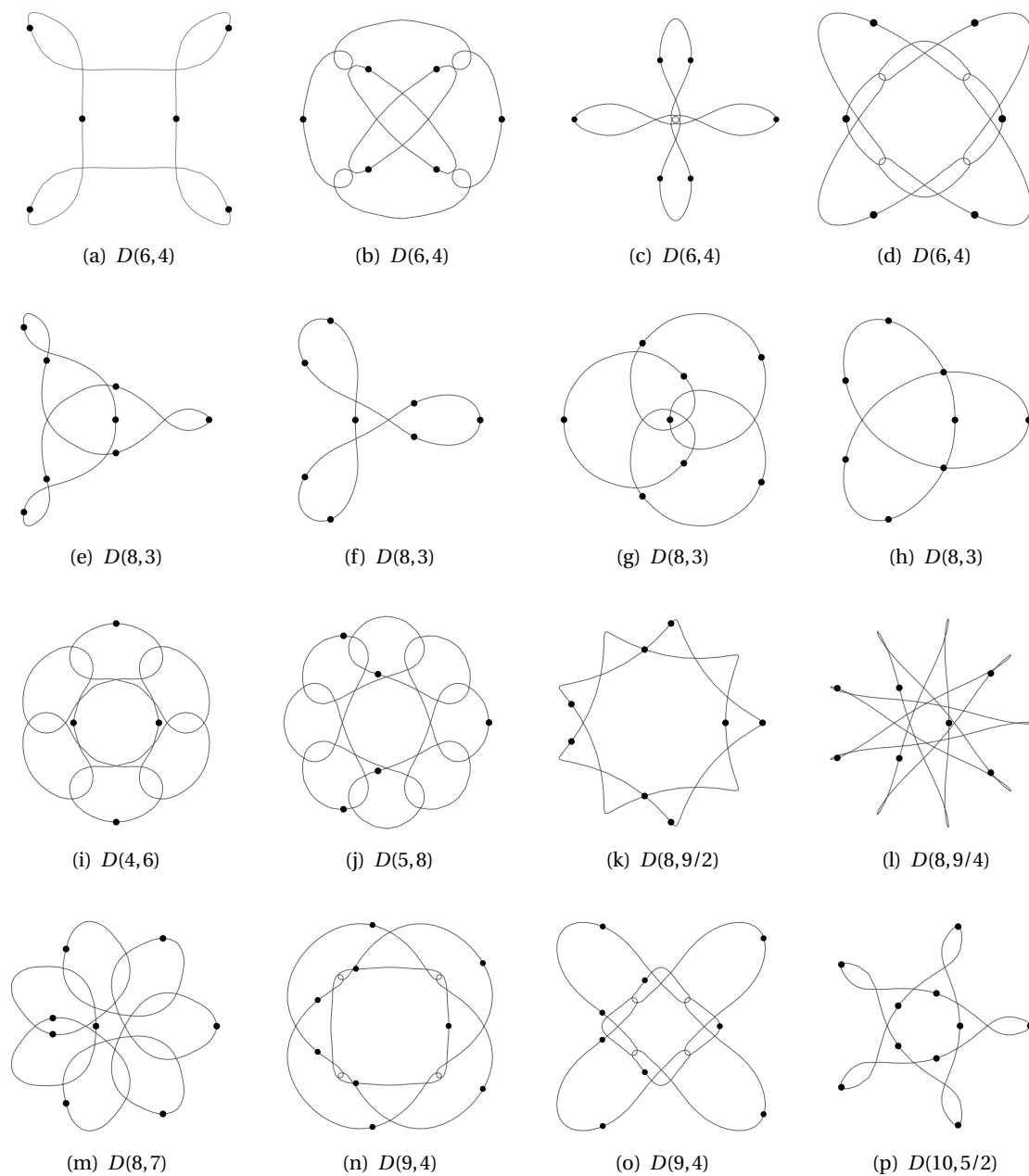
FIGURE 1.2: A selection of choreographies with their symmetry group. See Remark 1.6. These are all from the regular families of symmetry groups; for some examples illustrating the exceptional symmetry groups see Fig. 2.4. Where the same label appears for more than one figure, they correspond to different connected components of the corresponding \text{Fix}(G, \Lambda X^{(m)}) . Animations can be viewed on the first author's website [27].
