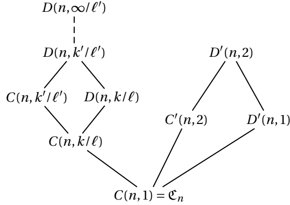
FIGURE 2.5: Lattice of isotropy subgroups, with k|k' and \ell' \equiv \pm\ell \pmod{k} .
