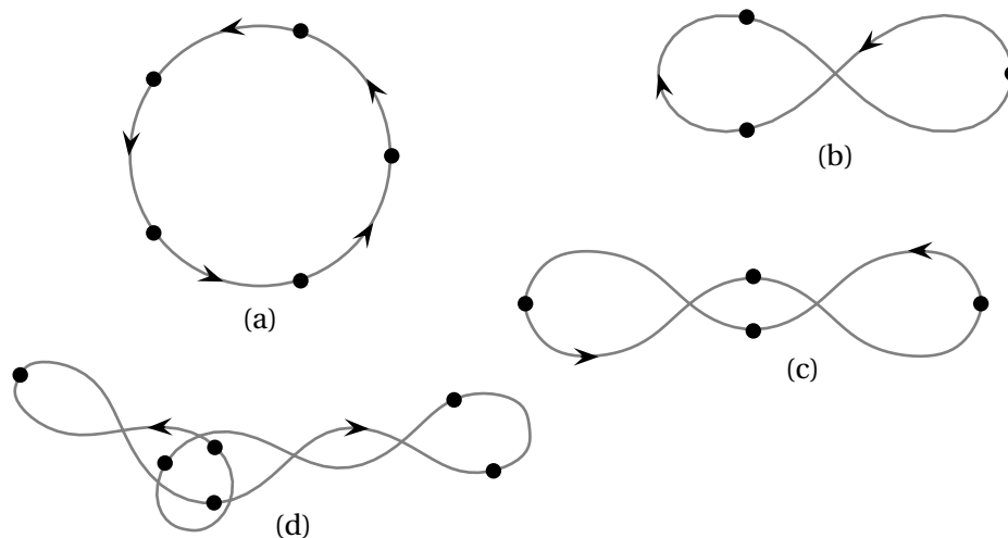
FIGURE 1.1: Examples of planar choreographies; (a) circular, (b) the figure eight, (c) the super-eight and (d) a non-symmetric choreography.
