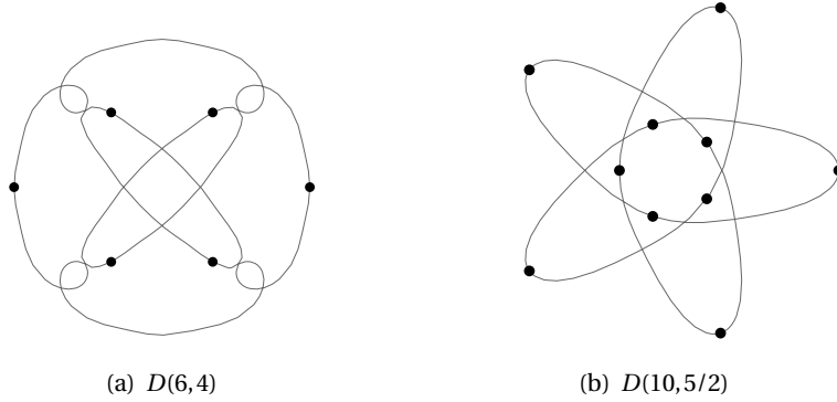
FIGURE 5.3: Two examples illustrating different connected components of each symmetry type compared with those in Figure 2.3, see also Remark 1.6. Many examples of 5-body choreographies with a single time-reversing reflectional symmetry—so type D(5,1) —in different connected components have been found (numerically) by Simó [35, Figure 3].
