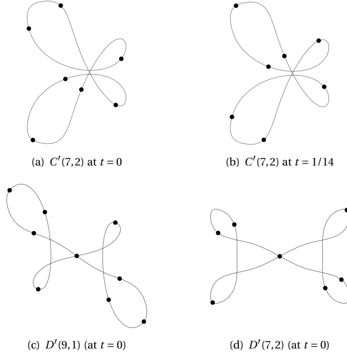
FIGURE 2.4: Exceptional symmetry groups. (a,b) A choreography for the 7-body problem, with symmetry C'(7,2) , demonstrating the symmetry generator (\kappa, \sigma_2, 1/14) , where here \sigma_2 = (1\ 5\ 2\ 6\ 3\ 7\ 4) . (c) A choreography with D'(9,1) symmetry: rotation by \pi is combined with a time reversal. (d) A choreography with D'(7,2) symmetry which possesses both the other symmetries: a rotation by \pi combined with time-reversal as well as a reflection which is not time reversing; another with this symmetry, in a different connected component, would be the figure-8 curve with 7 particles. See [27] for animations.
