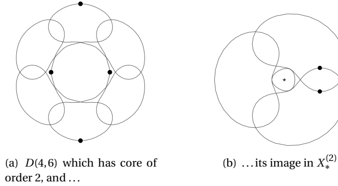
FIGURE 3.1: A choreography u for the 4-body problem with 6-fold symmetry, which has core of order 2, and its image \hat{u} under the map \Psi .
