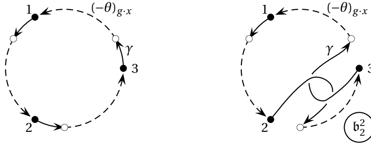
FIGURE 5.4: Two braids arising from loops with D(3,4) symmetry. The first is the circular choreography, the second the one depicted in Fig 2.2. The black dots represent the base point z_0 \in X^{(3)} , and the open dots the point \gamma(1) = g \cdot z_0 , where g = (R_{-\pi/2}, \sigma_1^{-1}) , and \sigma_1^{-1} = (1\ 3\ 2) . The solid curves represent \gamma and the dashed ones (-\theta)_{g \cdot x} . (A break in the solid path in the second figure represents the one traversed later: in other words this is a top-down view of the motion, with time increasing downwards and the ‘hidden’ curve broken as usual.)
