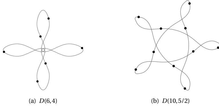
FIGURE 2.3: Two examples of choreographies with nontrivial core: in the first the order of the core is c = 2 and in the second c = 5 (generated by rotations through \pi and 2\pi/5 respectively). They are shown for generic values of t illustrating the core symmetry which is valid for all t . Compare with special configurations t = 0 in Fig. 1.2 (c) and (p)
