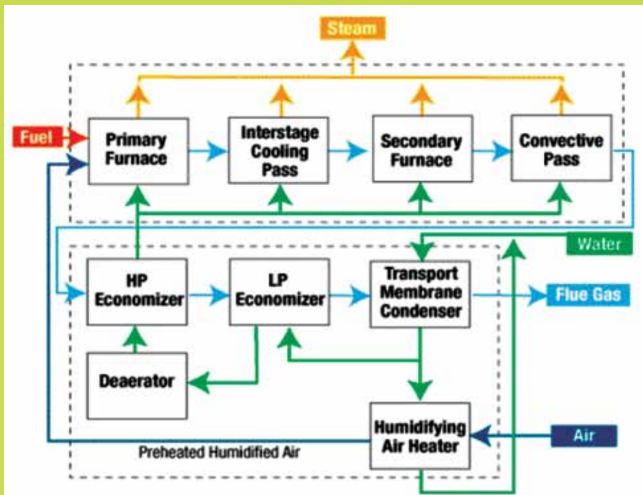
Figure 2: Two-stage Super Boiler [4]
