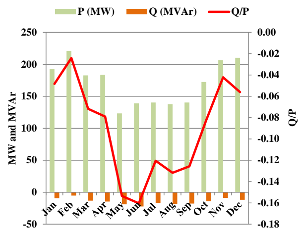
Fig. 3. Monthly analysis results for a GSP in South West of Great Britain for year 2012.
