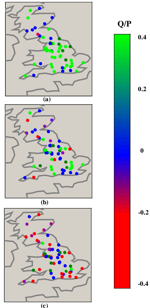
Fig. 1. Reactive power to active power ratios (Q/P ratios) during minimum load across Great Britain for a) year 2005, b) year 2010 and c) year 2012.
