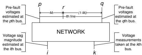
Fig. 1. A representation of the estimated and monitored buses required to perform fault location and voltage sag profile estimation. ( 1 column figure )
