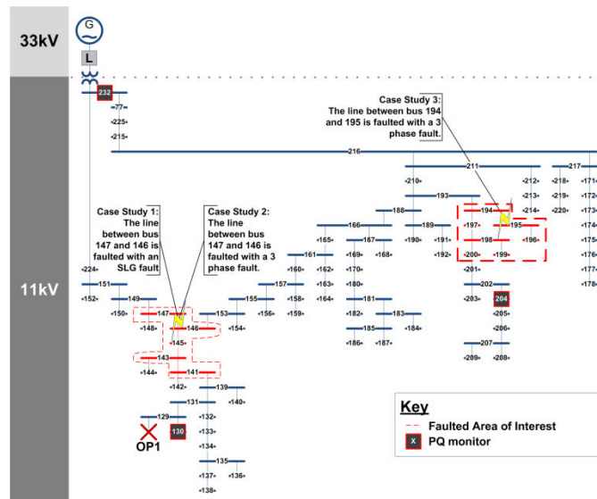
Fig. 2. 94 bus section of a 295 bus generic distribution network [23]. ( 1 column figure )
