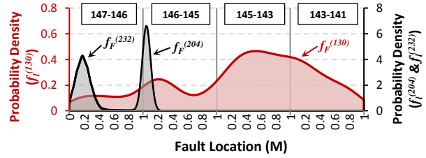
Fig. 11. The PDF of the fault location for a three phase fault: f_f^{(130)} , f_f^{(204)} , and f_f^{(232)} . (1 column figure)
