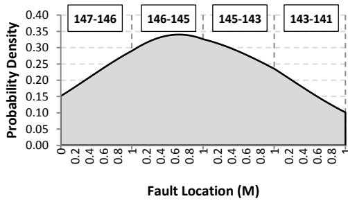
Fig. 6. The PDF for the fault location f_F^{(232)} . (1 column figure)
