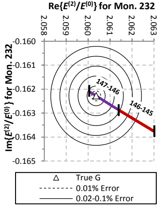
Fig. 3. Contours of constant G_{232} for errors in |E_{232}^{(2)}| and |E_{232}^{(0)}| . (1/2 column figure)
