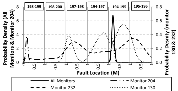
Fig. 15. The PDF across 6 lines for a three phase fault at 0.2 per unit along the line connecting bus 194 to bus 195 using all monitors ( f_f ) a monitor installed at bus 204 ( f_F^{(204)} ) 232 ( f_F^{(232)} ) and 130 ( f_F^{(130)} ). (1 column figure)
