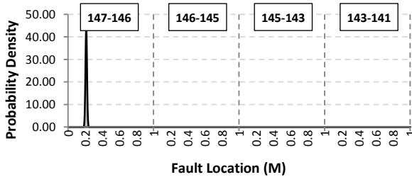
Fig. 8 The PDF of the fault location for a SLG fault: f_F^{(130)} ( f_F^{(204)} follows a very similar profile). (1 column figure)
