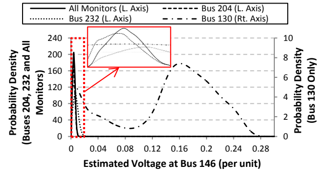
Fig. 13. The estimated probability distribution of the voltage magnitude in all three phases at bus 146 using measurements from bus 130, 204, 232 and all buses combined for a three phase fault. The inset shows a zoomed diagram of voltages less than 0.01 per unit. (1 column figure)
