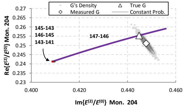
Fig. 9 The range of expected values for G_{204} . (1 column figure)
