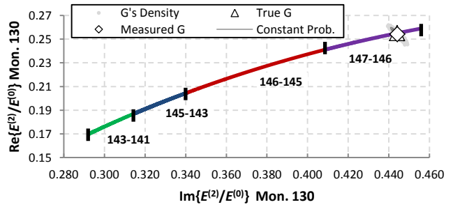
Fig. 7. The range of expected values for G_{130} . (1 column figure)
