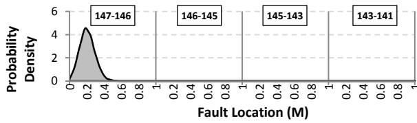
Fig. 12. The PDF of the fault location for a three phase fault: f_F . (1 column figure)
