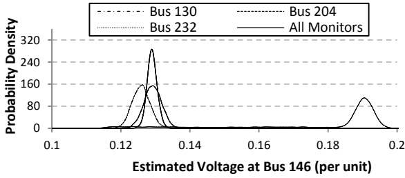
Fig. 10. The estimated probability distribution of the voltage magnitude in phase A at bus 146 using measurements from bus 130, 204, 232 and all buses combined for a single phase to ground fault. (1 column figure)
