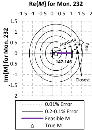
Fig. 4. The range of true and erroneous solutions for M_{147-146} given a constant error in |E_{232}^{(2)}| and |E_{232}^{(0)}| . (1/2 column figure)
