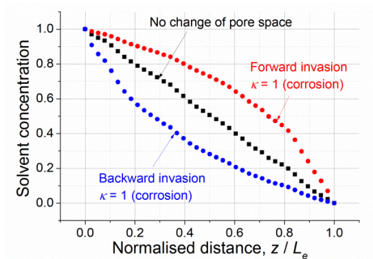
Fig. 5. Steady-state concentration profiles of solvent, U(VI), as predicted by the model with pore space changes due to corrosive agent diffusing in parallel with (forward) and opposite to (backward) solvent diffusion. Profile with no pore space changes shown for comparison.
