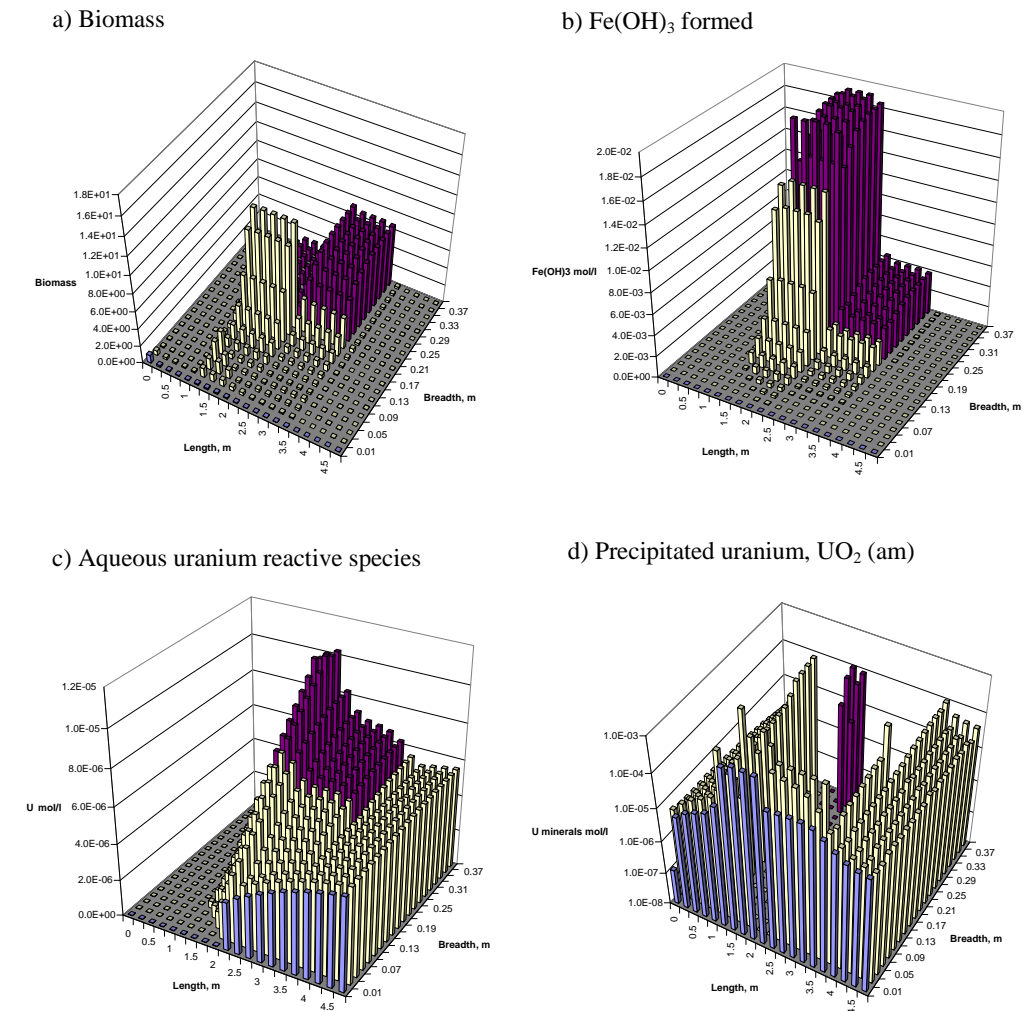
Fig. 8. Model results after 100 years for a lower effective diffusion coefficient D=2.2\text{E-}10\text{ m}^2/\text{s} , due to a 17.6% porosity decrease to 0.56.
