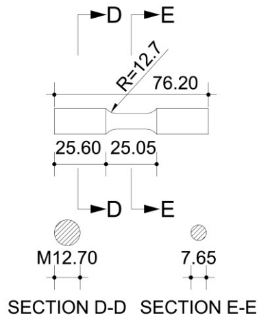
(b) tensile specimen (material 2)
