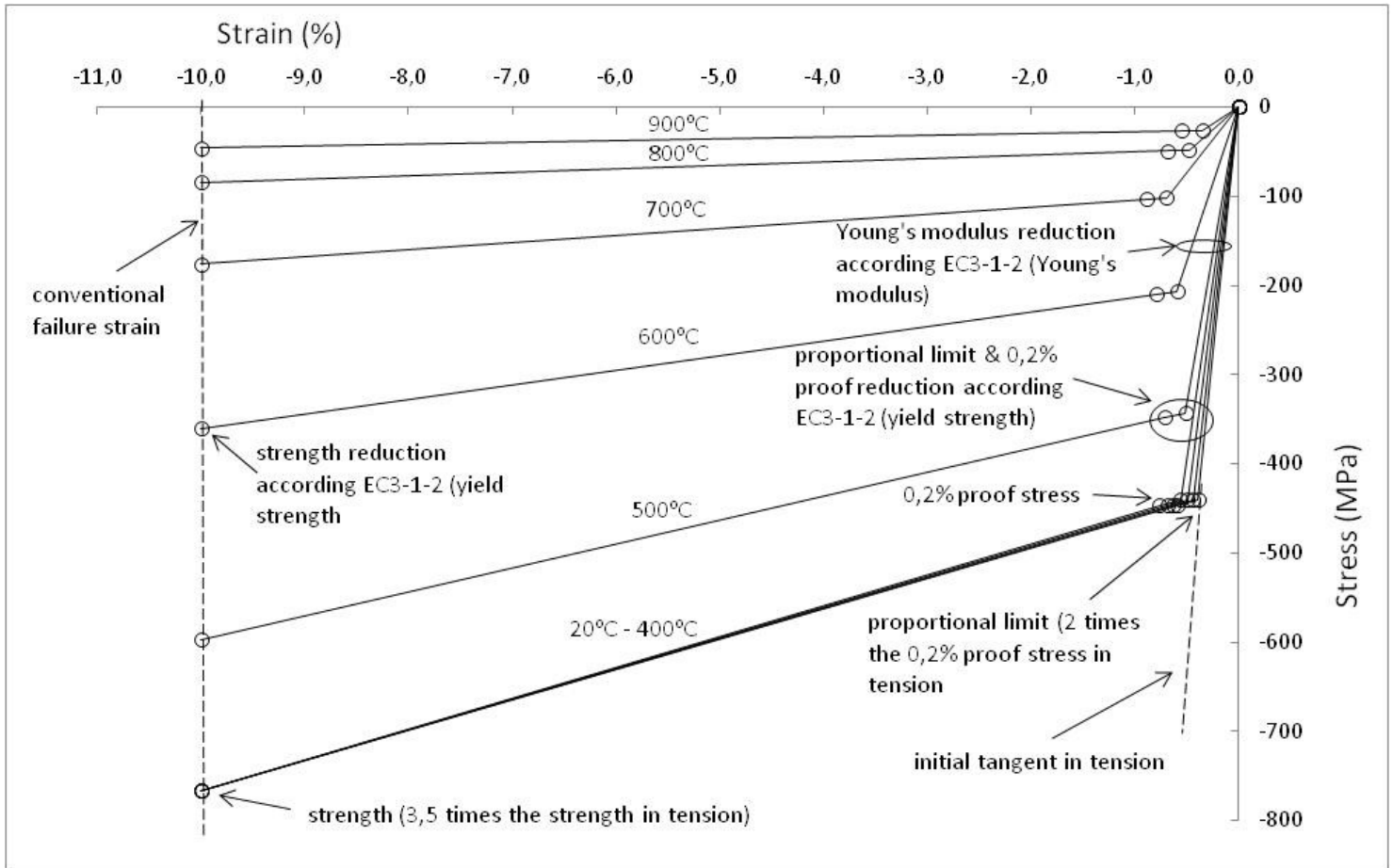
Figure 15 Proposed stress-strain relationships of cast iron in compression.
