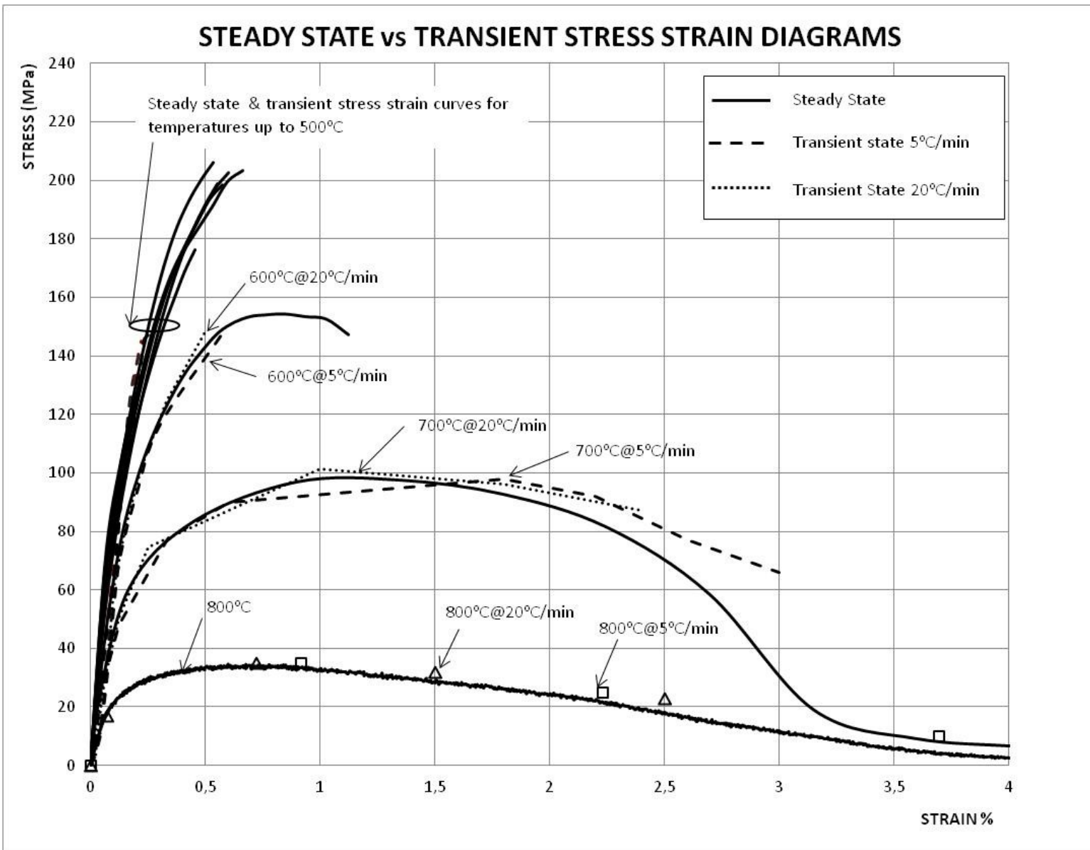
Figure 8: Comparison of stress-strain curves from the steady-state and transient state tests
