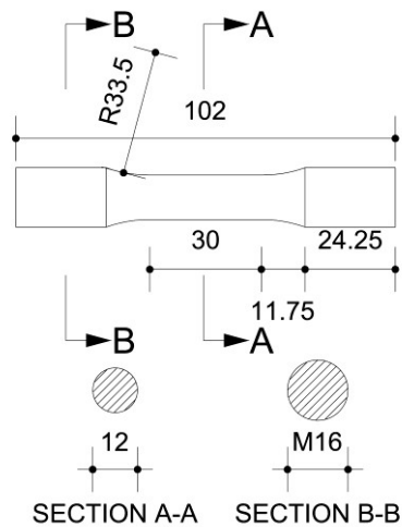
(a) tensile specimen (material 1)
