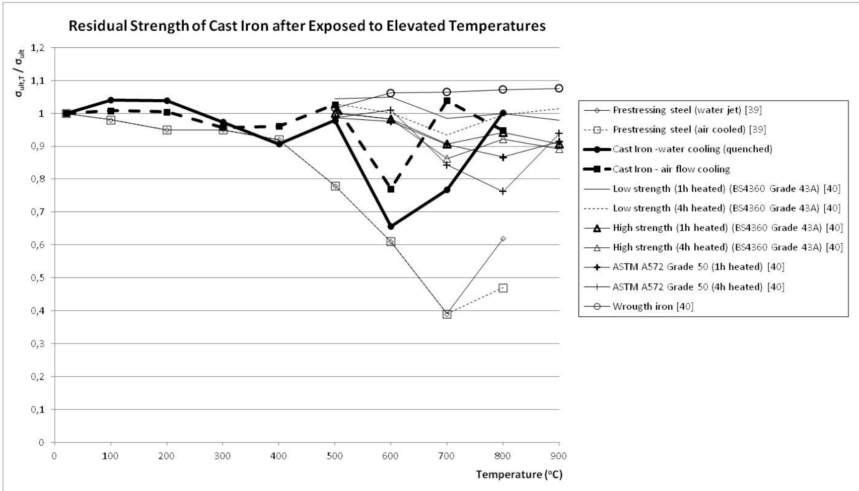
Figure 19. Comparison of residual strength of cast iron after exposure to elevated temperatures with those of wrought iron and structural and prestressing steels.
