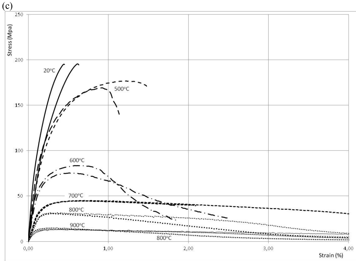
Figure 6: Steady state results under tension, (a) and (b) Group A tests, (c) Group E tests.
