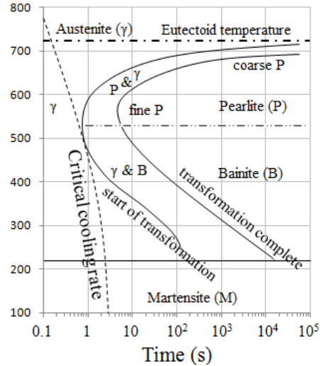
Figure 20: Schematic diagram illustrating isothermal curves (IT), critical cooling curves and resulting microstructures for eutectoid steel [42]
