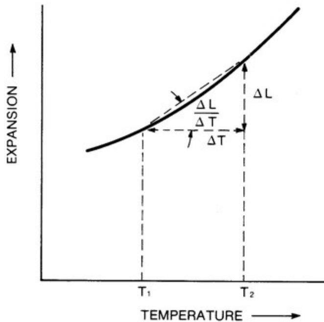
Figure 16: Calculation of thermal expansion [37]
