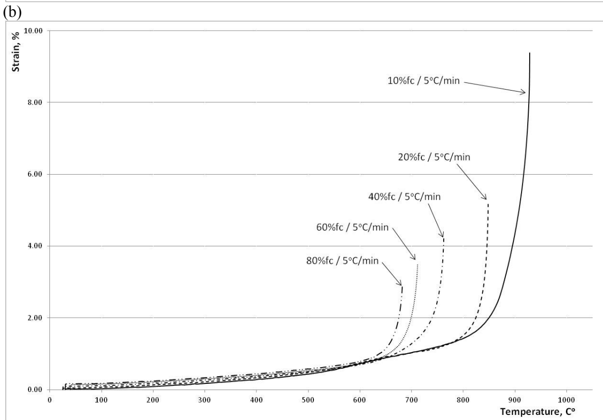
Figure 7: The effect of (a) heating rate and (b) of utilization factor from Group B transient tests.
