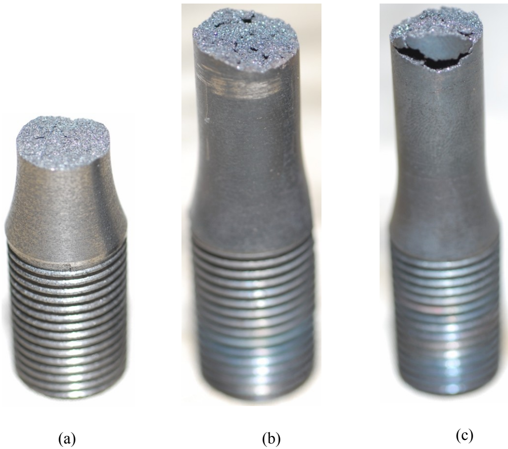
Figure 5: Different intergranular fracture modes in tension: (a) brittle failure at room temperature, (b) moderately brittle fracture at 700°C and (c) multi surface moderately brittle fracture at 700°C.
