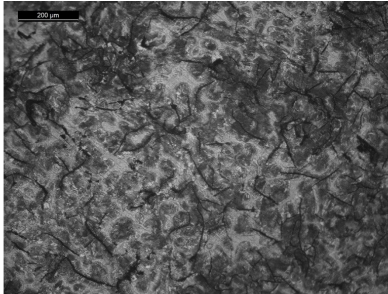
Figure 2: Microstructure of cast iron test specimens (200X (upper), 100X (lower))
