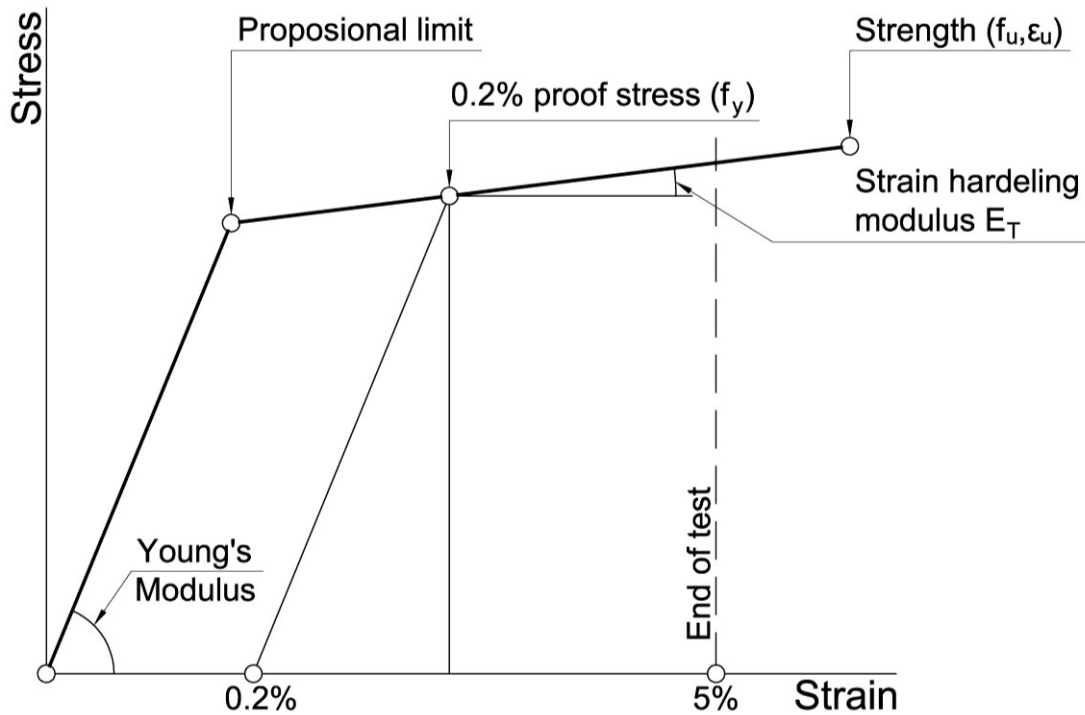
Figure 11: Typical stress-strain diagram of cast iron in compression
