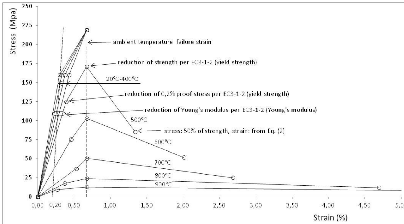
Figure 10. Proposed stress strain temperature relationship of cast iron in tension
