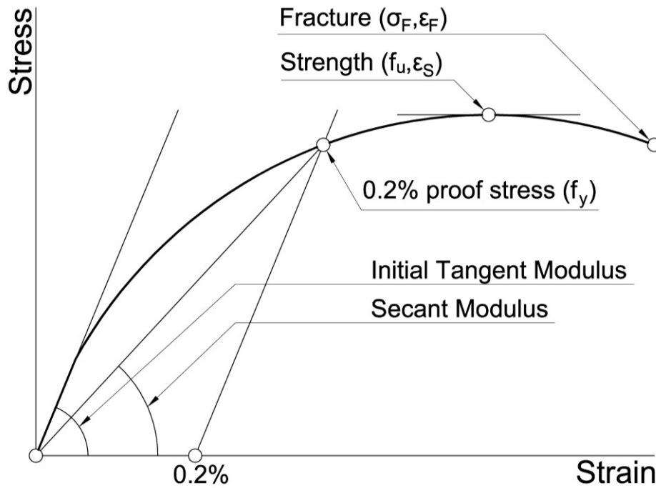
Figure 4: Typical stress-strain diagram of cast iron in tension
