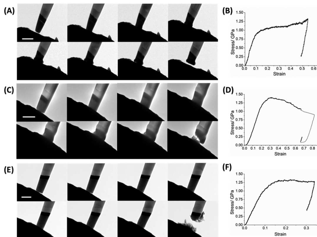
Figure 4. Time-lapse images of micromechanical compression tests; a stratified pillar of \text{MoS}_2\text{:Ni:SiO}_2\text{:Si} (bottom to top) of a diameter in the order of 100–500 nm is compressed at a constant rate of displacement by a Hysitron PicoIndenter tip during bright-field TEM imaging. The scale bars in all figures represent 500 nm and apply to all images. Frames are taken \sim 60 s apart from a continuous video. (a) Tip comprising \text{MoS}_2 , (b) typical stress/strain curve for \text{MoS}_2 , (c) tip comprising 10 at % Cr-doped \text{MoS}_2 , (d) typical stress/strain curve for 10 at % Cr-doped \text{MoS}_2 , (e) tip comprising 50 at % Cr-doped \text{MoS}_2 , (f) typical stress/strain curve for 50 at % Cr-doped \text{MoS}_2 .
