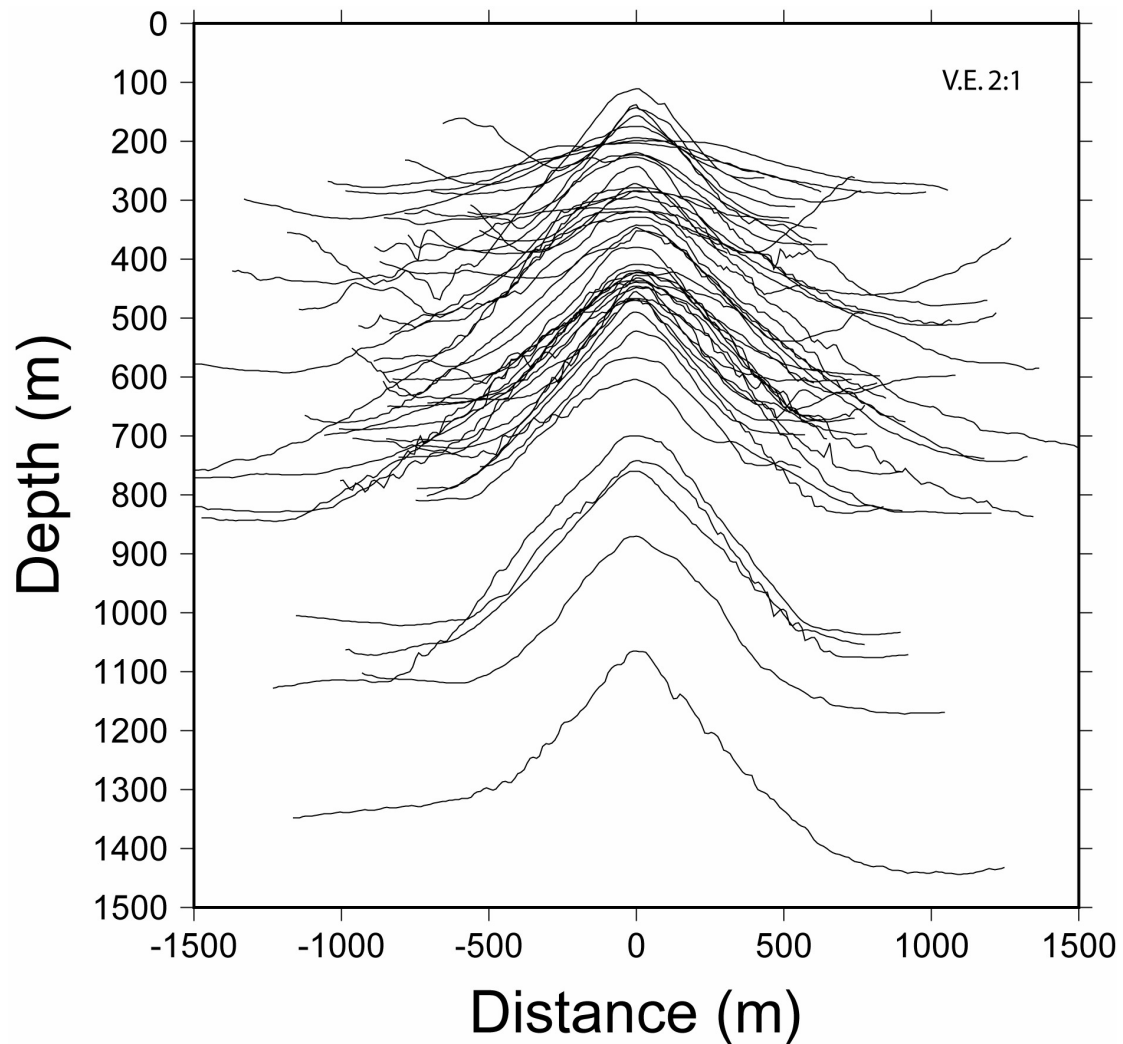
Figure 2. Bathymetry profiles of the submarine cones centred laterally according to their summit locations. Vertical exaggeration is 2:1.
