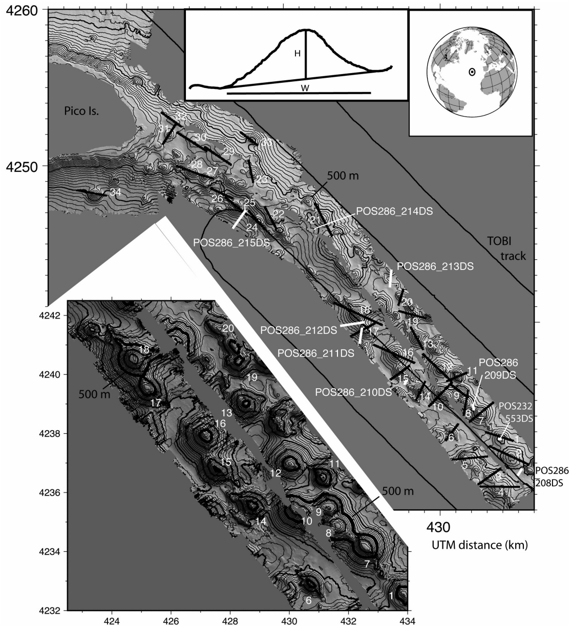
Figure 1. Multibeam echo-sounder dataset from the submarine ridge extending southeast of Pico Island. Bold black lines numbered with white lettering show where topographic cross-sections of cones were taken. Also shown are the sites of rock dredges (bold white lines annotated POS, etc) and the path of the TOBI deep-tow vehicle used in surveying the ridge in 1999 (Stretch et al. 2006) (solid line). Bathymetry data have been gridded at 25 m and contoured at 50 m (500 m intervals are shown in bold). Coordinates are Universal Transverse Mercator projection (zone 26) distances in km, which provide scale. Top-right inset
