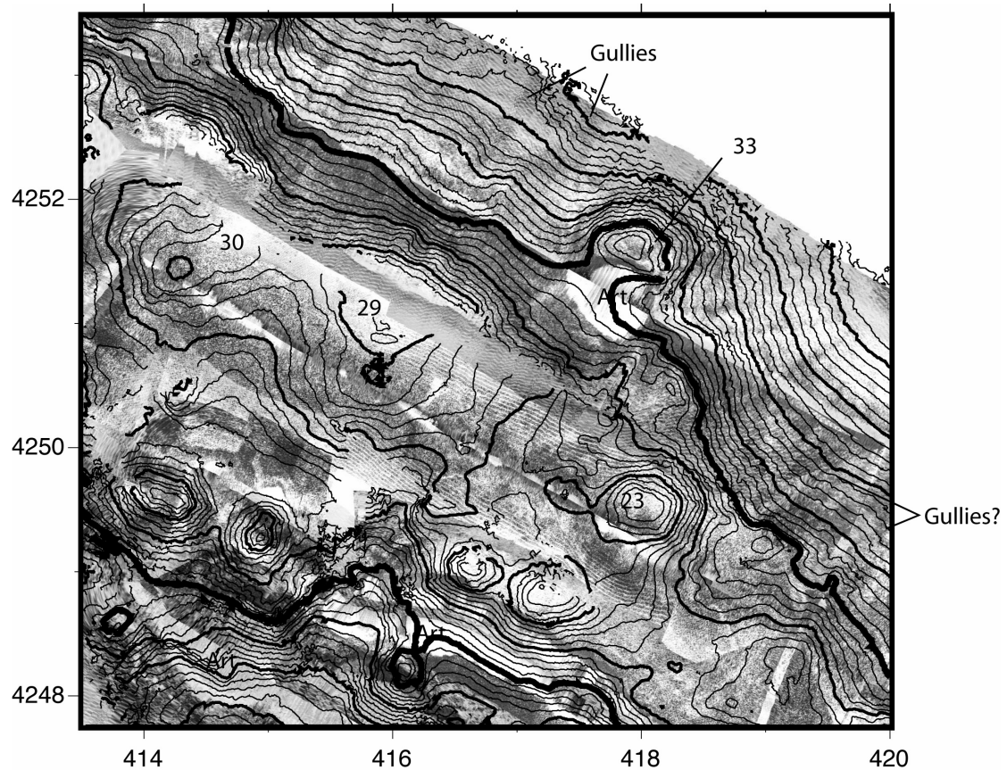
Figure 6. Acoustic backscattering mosaic derived from the multibeam sonar data (high backscattering shown with dark tone). Cone numbers correspond with those in Figure 5 (inset), which includes the bounds of the map. Note smooth texture under cones 29 and 30.
