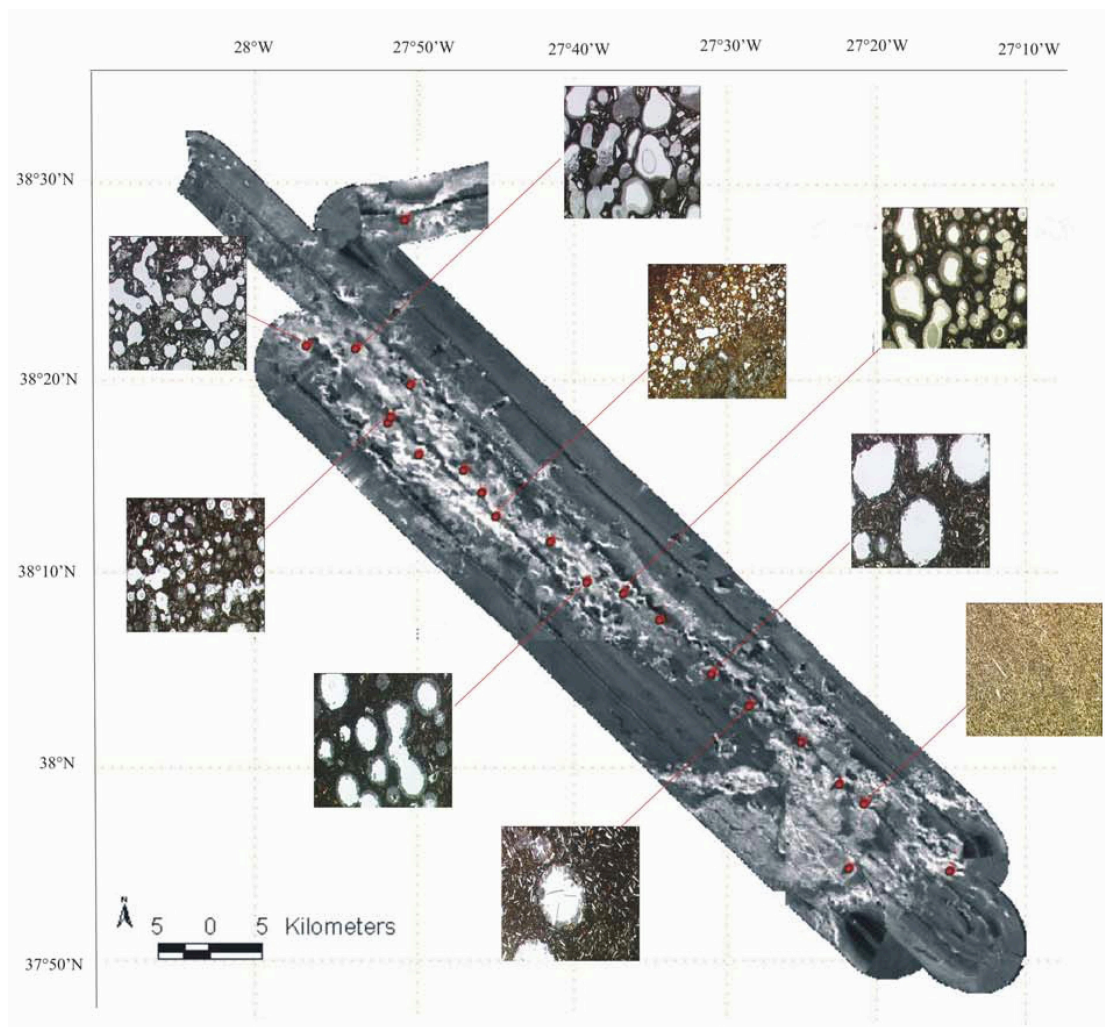
Figure 7. Thin section images of dredge samples collected on R/V Poseidon cruises 232 and 286. Background is a greyscale map of TOBI deep-tow sidescan sonar data (Stretch et al. 2006). White represents high backscatter. Thin section images are about 5 mm across.
