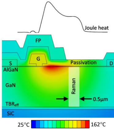
Fig. 3: Combined drift diffusion and 3D finite element thermal modelling result, showing a temperature cross section through a packaged two finger AlGaIn/GaN-on-SiC HEMT (half the device is shown) operated at 50V_{DS} , -1.5V_{GS} and a power dissipation density of 11 \text{ W/mm}^2 , at 25^\circ\text{C} ambient temperature. The Joule heating profile in the 2DEG channel is shown above for visual reference. The model is adapted from [4].
