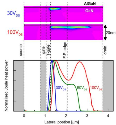
Fig. 9: Simulated channel heating distribution map of AlGaIn/GaN-on-SiC HEMT with field plates at different drain bias voltages. Reprinted from [4], Copyright 2015, with permission from Elsevier.
