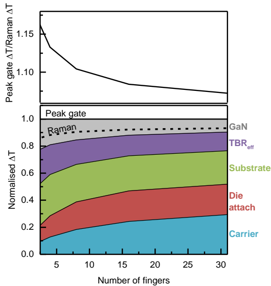
Fig. 8: Simulated temperature rise in a packaged GaN HEMT on a 100\mu\text{m} -thick SiC substrate, shown as a function of number of gate fingers at a constant power dissipation density of 11\text{W}/\text{mm} ; using a model adapted from [4]. The ratio between the peak gate temperature rise and spatially averaged temperature rise, equivalent to a Raman thermography measurement, is shown. The temperature across each layer in the device stack is also shown, normalized to the peak gate temperature. A eutectic die attach and CuW carrier are included, representing the package.
