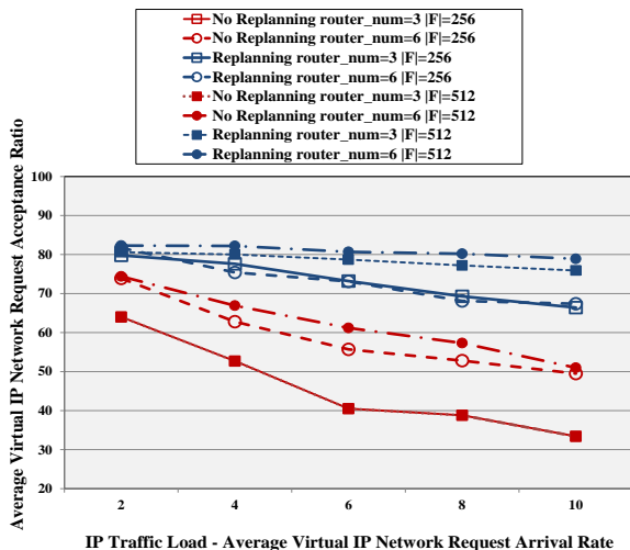
Fig. 12. Average VIPN request acceptance ratio for varied router_num and |F|
