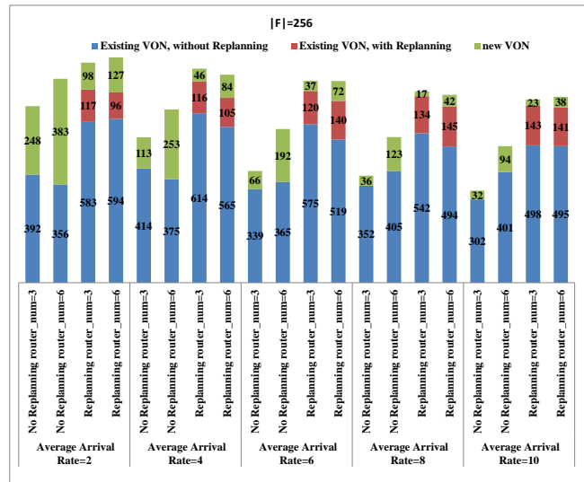
Fig. 14. Comparison of the utilization of VONs during the composition of VIPNs ( |F|=256 )
