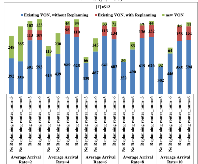
Fig. 15. Comparison of the utilization of VONs during the composition of VIPNs ( |F|=512 )
