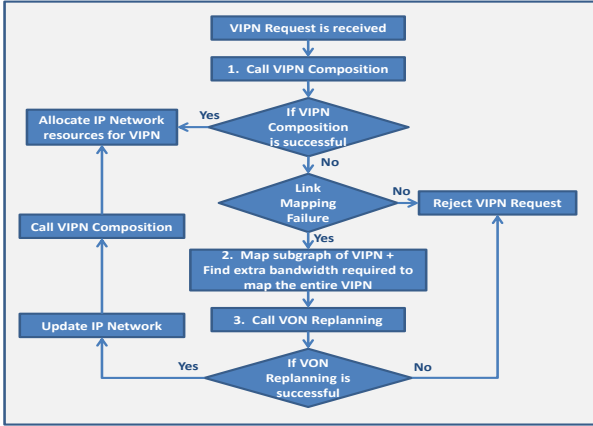
Fig. 3. VIPN Composition coordinated with VON Replanning
