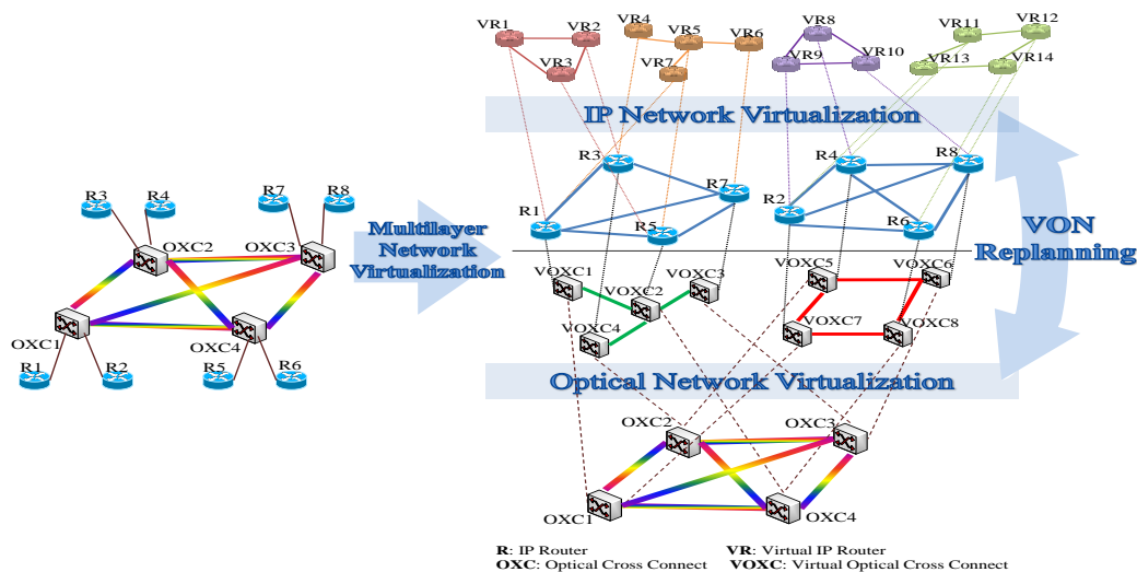
Fig. 1. Network Virtualization in IP over Optical Network
