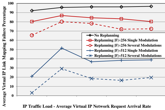
Fig. 9. Average percentage of link mapping failure for varied |F| and different support modulations
