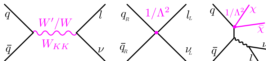
FIG. 1 (color online). Production and decay of an SSM W' or W_{KK} -boson (left), HNC-CI (center), DM single W -boson production (right).
