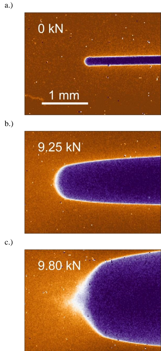
Figure 5: X-ray images of the notch tip of Specimen 2 under the different loading states shown in Figure 2. a.) The semi-circular tip of the initial EDM notch, b.) blunting of the notch during loading and c.) initiation of ductile tearing.
