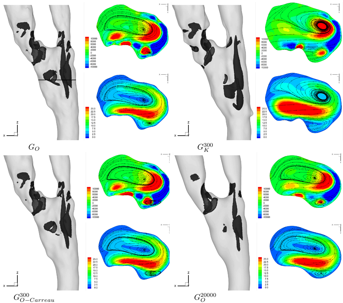
Figure 13. Q=10000 iso-surfaces and cross sections showing Q (top), the velocity magnitude ( \text{m s}^{-1} ) (bottom) and in plane particle trajectories, for a selection of the cases studied. Top left insert shows the cross section location.
