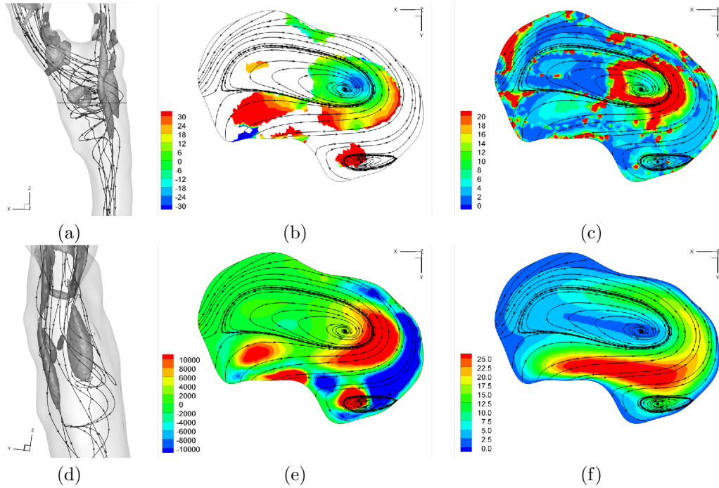
Figure 11. Result for G_O^{300} and Newtonian fluid. Passive particle track and iso-contours of Q=10000 viewed in-plane (a) and from the anastomosis ‘floor’ (d). Discernible is the jet from the graft that impinges on the anastomosis ‘floor’, which divides the flow due to the relative planarity of the vessel bifurcations to form two counter rotating vortices. Cross section (location shown in (a)) of: (b) magnitude of \lambda_1 for complex eigenvalues of the velocity gradient tensor (regions where the eigenvalues are all real a coloured white); (c) |\lambda_3/\lambda_2| to indicate the spiralling compactness (for a foci configuration as indicated for regions shown in (b)); (e) Q (the second invariant of the velocity gradient tensor) (f) velocity magnitude ( \text{m s}^{-1} ).
