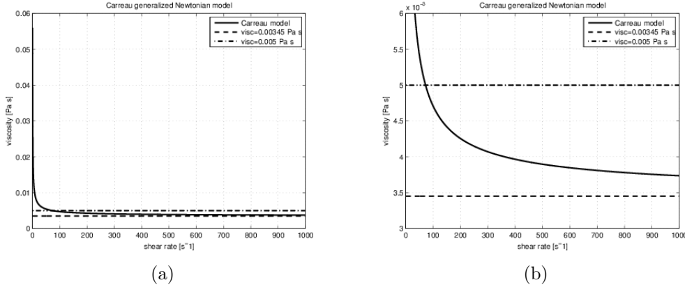
Figure 8. Varying viscosity ( Pa\ s ) with the shear rate ( s^{-1} ) in the Carreau shear-thinning model, showing asymptotic behaviour (a) and detail (b).
