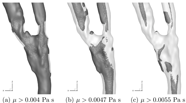
Figure 7. For G_{O-Carreau}^{300} , regions indicated are where the apparent viscosity calculated from the Carreau model used is greater than (a) 0.004, (b) 0.0047, and (c) 0.0055 Pa s. Note that regions identified in (b) correspond to low shear rates with \dot{\gamma} < 100s^{-1} .
