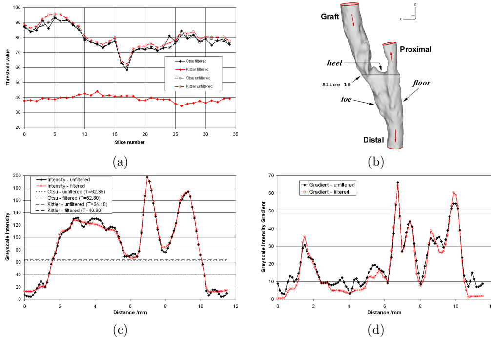
Figure 1. (a) Threshold variation along the image stack, where slice 0 corresponds to the distal extremity and between slice 16 and 17 lies the bifurcation to the bypass and proximal conduits. Location of slice 16 and nomenclature are shown in (b), as well as the flow direction. Variation of image intensity (c) and intensity gradient (d) are along the blue line shown in Figure 2 (going from bottom right to top left).
