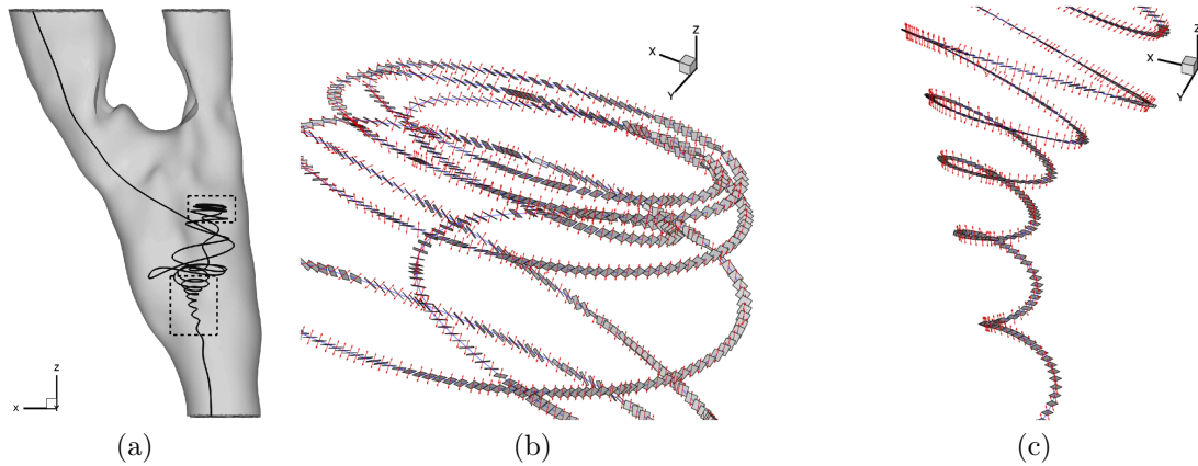
Figure 9. (a) Graft and passive particle track and (b), (c) detail of the trajectory in a vortical structure where the solution is \lambda_1, \lambda_2 \pm i\lambda_3 . Plane of swirling and axis of stretching are indicated, given by the eigenvectors of the velocity gradient tensor. It should be noted that for these details the foci are stable and \lambda_1 > 0 .
