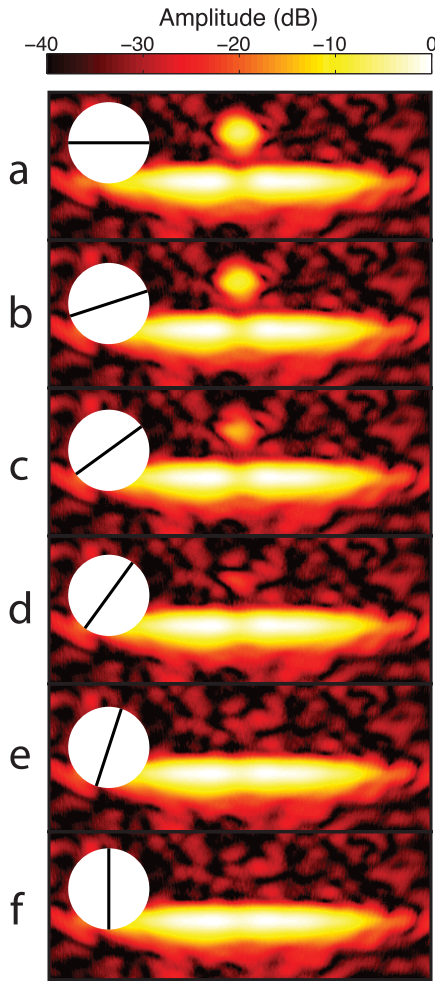
Fig. 8. TFM images for a 1-mm ( 0.71\lambda ) crack located 5 mm from the back wall of a 65-mm-deep specimen inclined at (a) 0^\circ , (b) 18^\circ , (c) 36^\circ , (d) 54^\circ , (e) 72^\circ , and (f) 90^\circ anticlockwise from horizontal with a crack angle schematic inset. The same array and filter as Fig. 5 has been used.
