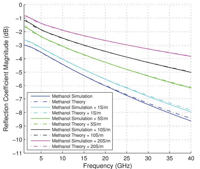
Fig. 6 Comparison of Frequency domain reflection coefficient of vacuum/methanol interface as found via the ETD stabilized Debye pole, with varying amounts of additive static conductivity. Theoretical response denoted by dashed line, FDTD simulation by solid line.
