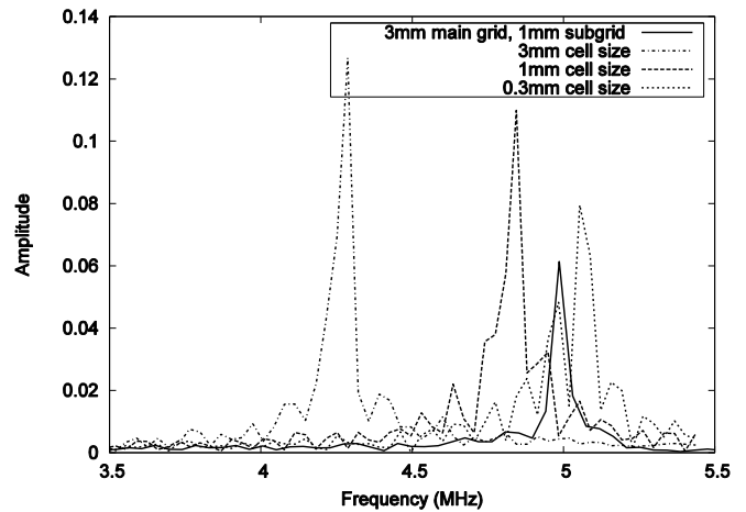
Figure 3 - Fourier Transform of the fields in the resonant cavity
