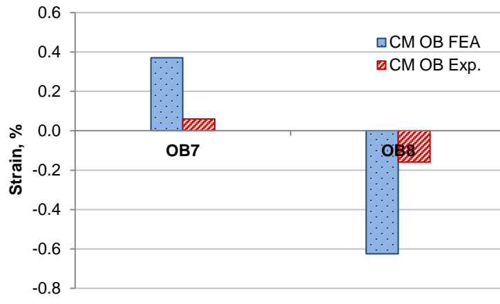
c) Outboard compliant mechanism results.
