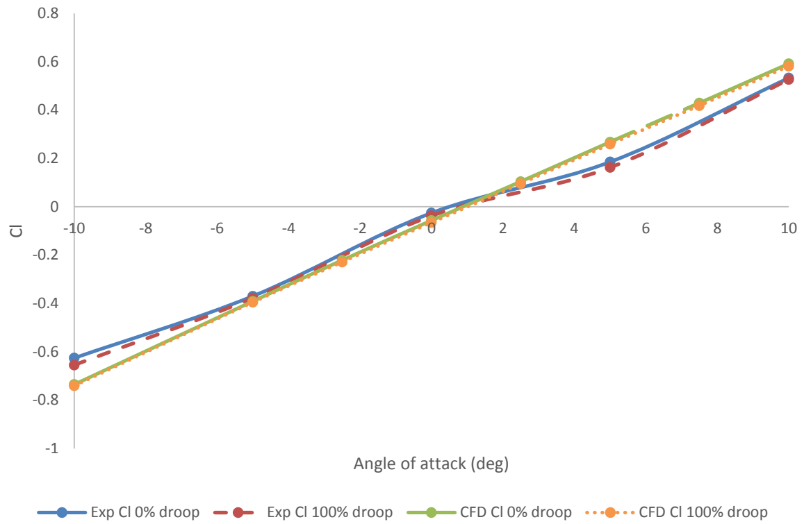
Fig. 12 Comparison of experimental and CFD lift coefficients at 55m/s.
