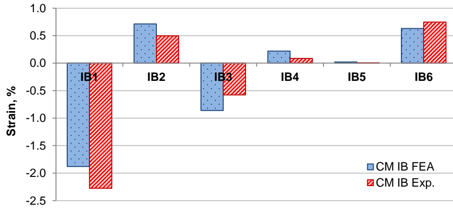
b) Inboard compliant mechanism results.
