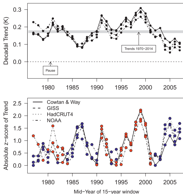
FIG. 1. Summary of all possible 15-yr trends in GMST between 1970 and 2014 inclusive. (top) The trend (K decade -1 ) for the 15-yr window centered on the plotted year for four datasets: NASA’s GISS (Hansen et al. 2010; http://data.giss.nasa.gov/gistemp/ , accessed 17 Jan 2015), the Met Office’s HadCRUT4 (Morice et al. 2012; www.metoffice.gov.uk/hadobs/hadcrut4/data/current/time_series/HadCRUT.4.3.0.0.annual_ns_avg.txt , accessed 2 Feb 2015), the coverage-bias-corrected version of HadCRUT4 reported by Cowtan and Way (2014) ( http://www-users.york.ac.uk/~kdc3/papers/coverage2013/series.html , accessed 2 Feb 2015), and the latest NOAA dataset (Karl et al. 2015; www.ncdc.noaa.gov/cag/time-series/global/globe/land_ocean/ytd/12/1880-2014.csv , accessed 12 Aug 2015). The GISS dataset is based on sea surface temperature data [Extended Reconstructed SST version 3b (ERSSTv3b)]. The decadal temperature increase is greater than zero (dashed horizontal line) in all datasets at all times. The gray horizontal band represents the average of the trends between 1970 and 2014 across the four datasets. The longer-term trend is represented as a band to capture some of the uncertainty from dataset to dataset, but also to indicate that this is an inherently imprecise quantity because it varies with the exact period that is chosen to represent a longer-term trend. (bottom) The same data as in the top panel, but 15-yr trends are converted into absolute z scores, by expressing each observed trend as the absolute difference in standard deviation units from the mean of all trends since 1970. Originally positive z scores (representing greater than average warming) are plotted in red, and originally negative z scores are shown in blue.
