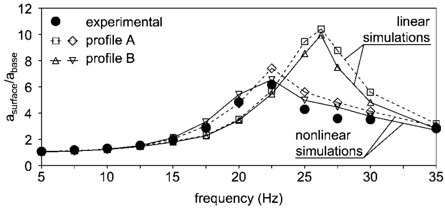
Fig. 21. Effect of soil nonlinearity on free-field surface acceleration for sine dwell excitation of variable frequency; a_{base} \approx 0.03g .
