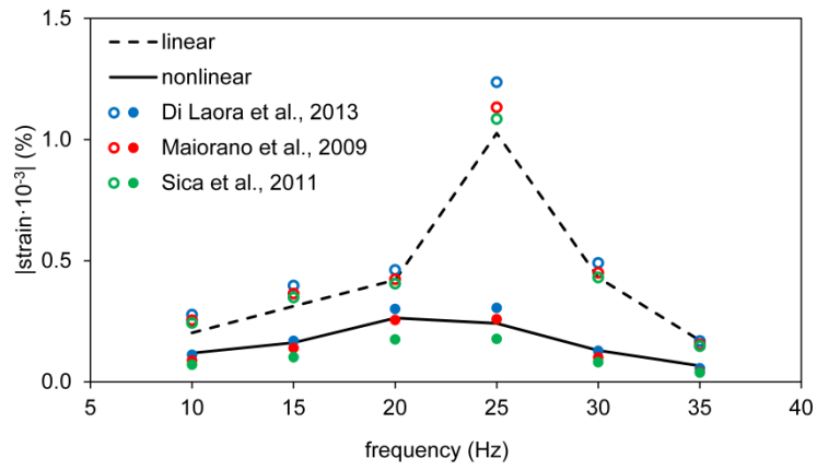
Fig. 25. Kinematic bending strain at the layer interface: comparisons between the present approach and simplified expressions; a_{base} \approx 0.03g .
