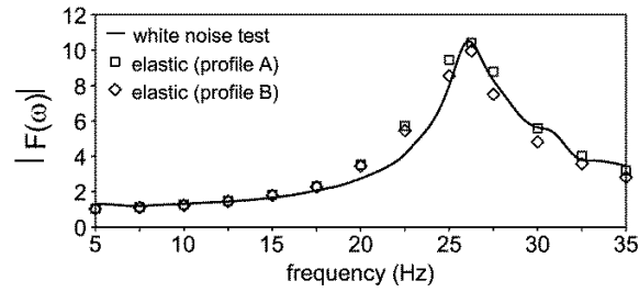
Fig. 16. Calculated linear amplification functions for profiles A and B, and experimental data for white noise test 101116_X1; a_{base}=0.02g .
