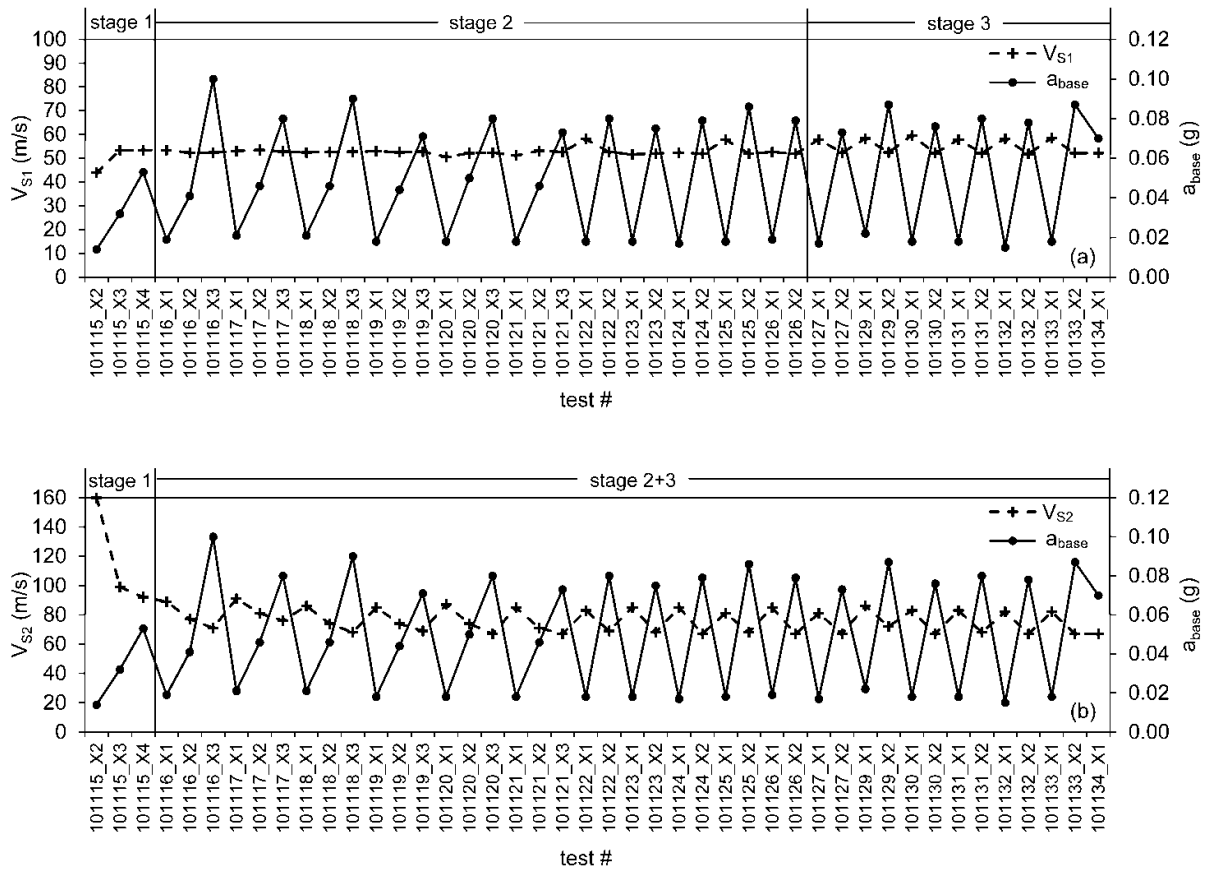
Fig. 9. Back-calculated fit shear wave velocities at top layer (a) and bottom layer (b) during white noise tests. Input acceleration level is shown on the right.
