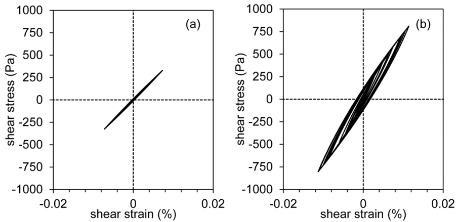
Fig. 22. Hysteretic loops at middle points of upper layer (a) and bottom layer (b) for sine dwell excitation, f=25 Hz, a_{base} \approx 0.03g
