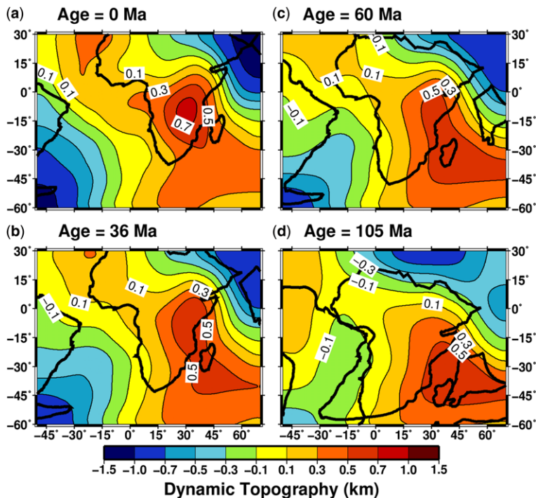
Fig. 4. Dynamic topography (in km) of Africa over the past 105 Ma (from Conrad & Gurnis 2003).
