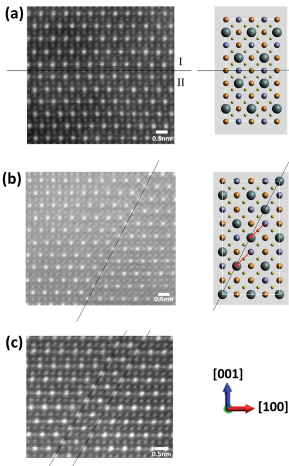
Fig. 3 Atomic resolution HAADF images of antisite domain boundaries (ADBs) showing fault displacement of \frac{1}{2}[110] (a), -\frac{1}{4}[201] (b) and -\frac{1}{2}[201] (c).
