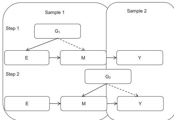
Figure 6. Schematic diagram of two-step, two-sample Mendelian randomization. In the smaller Sample 1, the association of the exposure to the intermediate is established using an MR approach (using the exposure-related G_1 ); and the association of an additional variant ( G_2 , not related to the exposure) with the same intermediate is established. G_1 and G_2 should be identified in an independent study. In the larger Sample 2, the intermediate is shown to influence the outcome through the use of G_2 , which is related to the outcome. N.B. the dotted arrows represent the fact that these genetic variants, G_1 and G_2 , influence the intermediate or outcome indirectly through the exposure or intermediate, rather than having a pleiotropic effect. In theory, G_1 would also be found to influence the outcome indirectly through both the exposure and intermediate.
