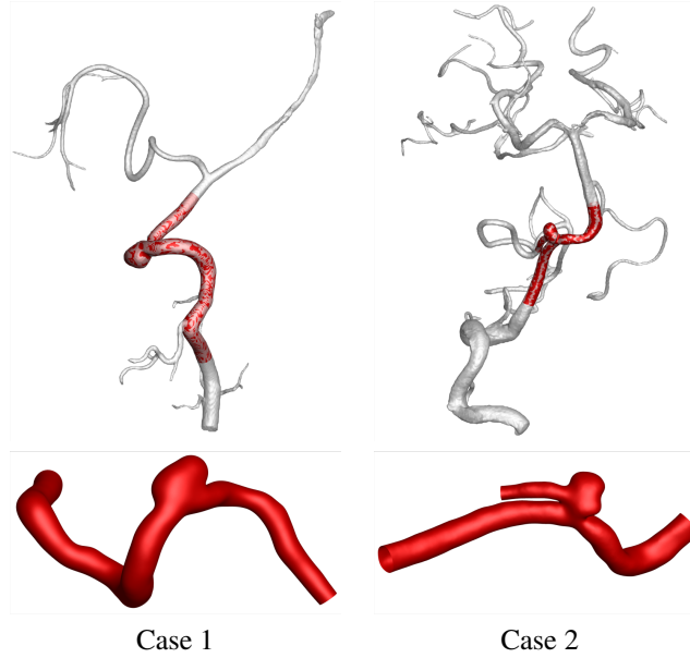
Figure 1: Top row: region of segmented cerebral vasculature and region of interest containing the aneurysm (flow is from bottom to top) for two patient data sets. Bottom row: detail of region of interest used as computational domain (flow is from left to right).
