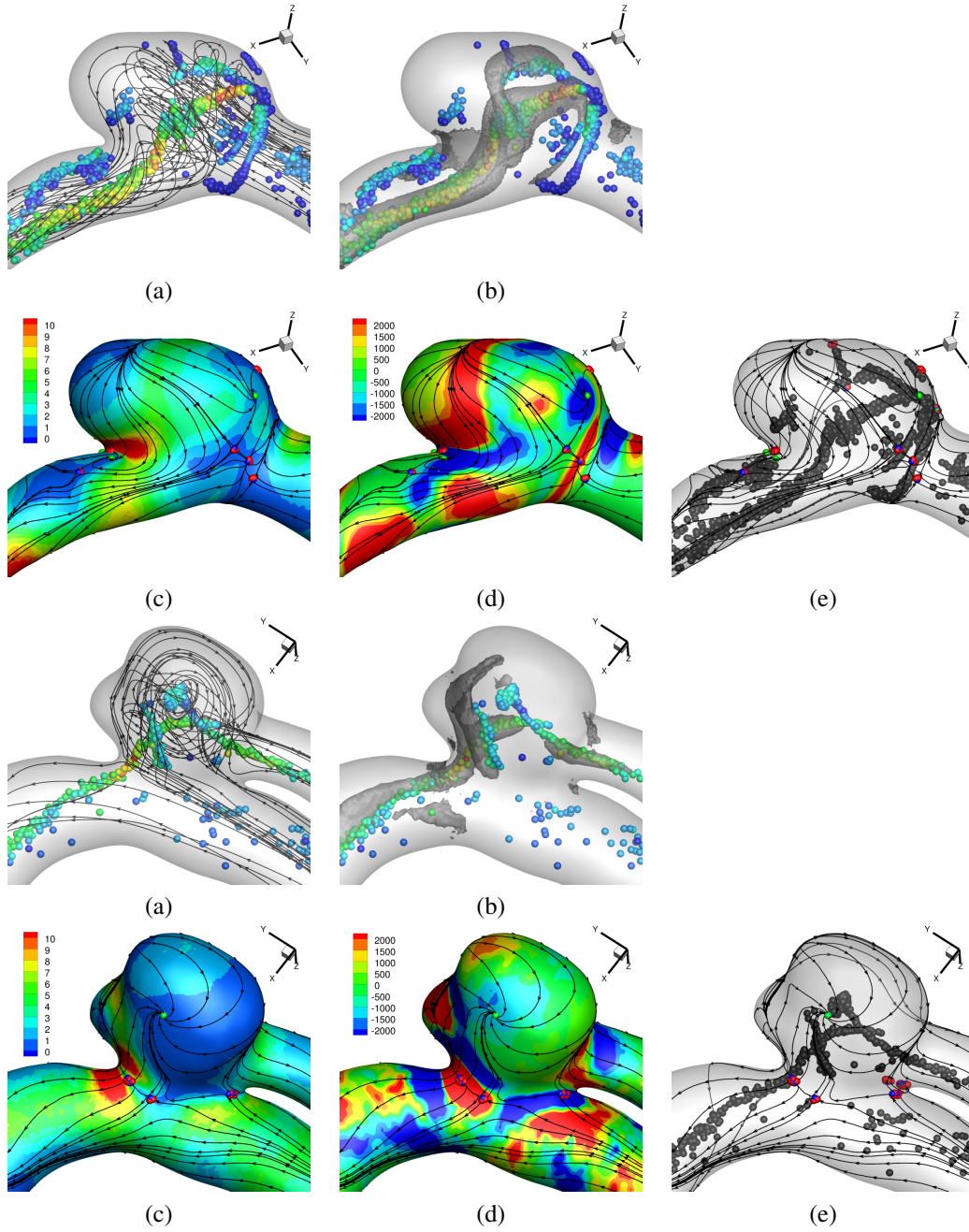
Figure 5: Steady-state computations for Case 1 (top) and Case 2 (bottom). (a) Streamlines and vortex core points coloured by the magnitude of the complex eigenvalue ( \lambda_3 ) of the velocity gradient tensor, hence the rate swirling. (b) Vortex core points and iso-surfaces of \lambda_2 = -10^4 for vortex identification [34]. Plots of surface shear lines and WSS critical points (same colouring scheme as in Figure 3) and (c) plot of WSS (/Pa), (d) TR (/Pa m -1 ), (e) vortex core points.
