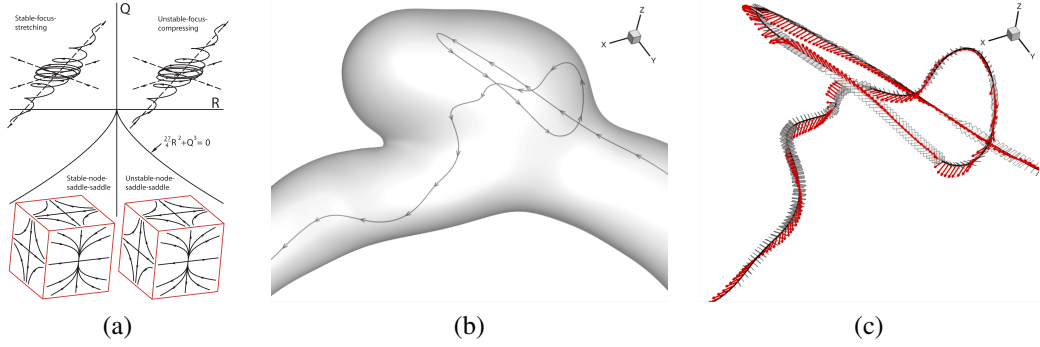
Figure 2: (a) Solution trajectories can be either node-saddle-saddle or focus-stretching, as well as either stable or unstable. The axes are the eigenvectors of the velocity gradient tensor. (b) Sample trajectory for steady-state computations of patient Case 1 and (c) region detail of trajectory in a vortical structure showing the plane of swirling and the axis of stretching, given by the eigenvectors of the velocity gradient tensor.
