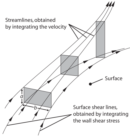
Figure 4: Surface shear lines, obtained by integrating the traction force components on the wall, coalesce (or diverge) and due to continuity the fluid moves away (or towards) the wall gradually, such that a \propto (b\tau_w)^{-1/2} , from equation 7, where \tau_w is the wall shear stress magnitude.
