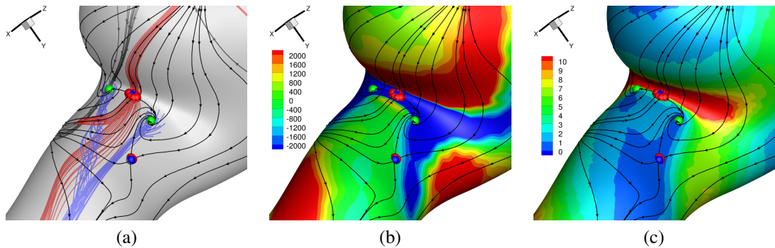
Figure 3: Detail of distal aneurysm neck region of steady-state computations for Case 1. The images show surface shear lines and WSS critical points, which are coloured such that green indicates a complex conjugate pair solution (spiralling motion), blue indicates real solutions and red are locations a small distance along the eigenvectors (hence principal directions). (a) Passive particle streamlines in the fluid domain indicate flow separation (red) and vortex cores touching the wall (blue) which are also identified by the WSS critical points. (b) Plot of TR ( \text{Pa m}^{-1} ) as the convective transport normal where positive values indicate flow movement to the wall and negative is movement away from the wall. The region of flow separation is marked as strong movement away from the wall for example. (c) Plot of WSS ( \text{Pa} ) and describes the convective transport parallel to the wall.
