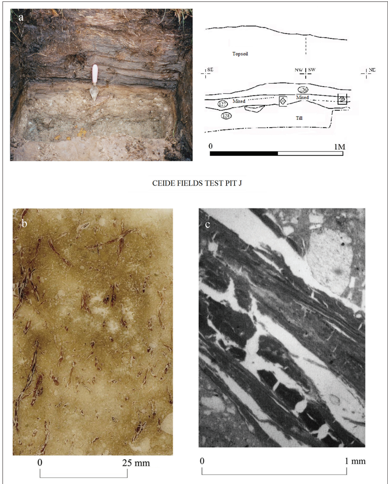
Figure 3. (a) Test pit J (Céide Fields) photo and section drawing; (b) Rootlets in the buried soil, macro (Céide Fields Test Pit I, layer 119); (c) Rootlets in the buried soil, micro (Céide Fields Test Pit I, layer 119).
